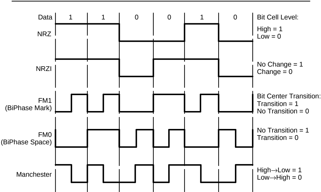
Figure 5–4. Data Encoding
