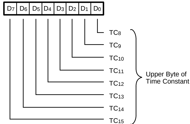
Figure 6–15. Write Register 13
