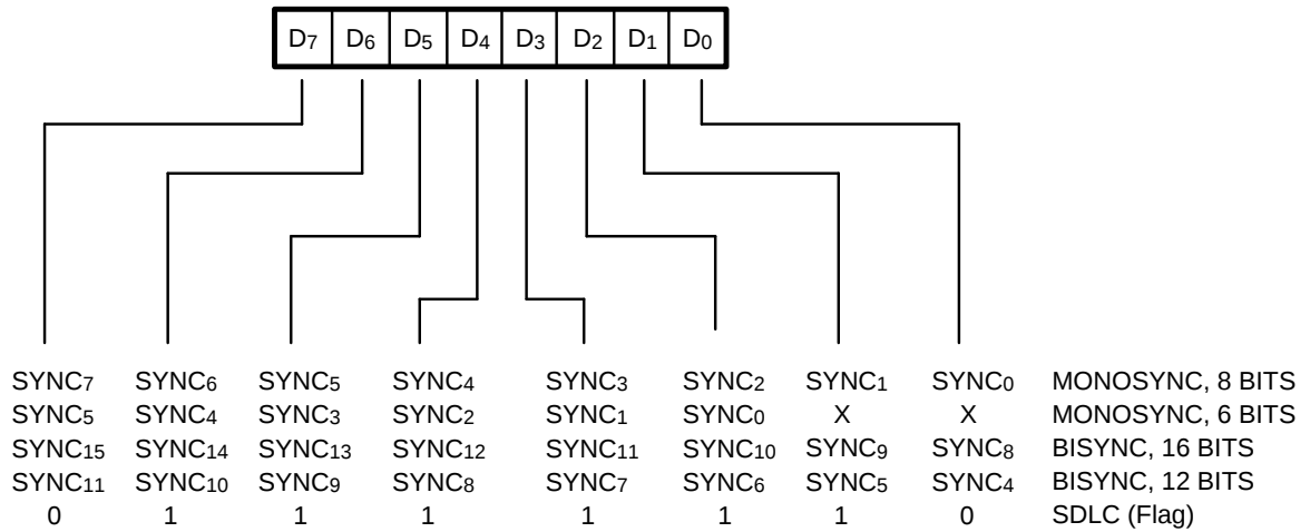
Figure 6-8. Write Register 7
