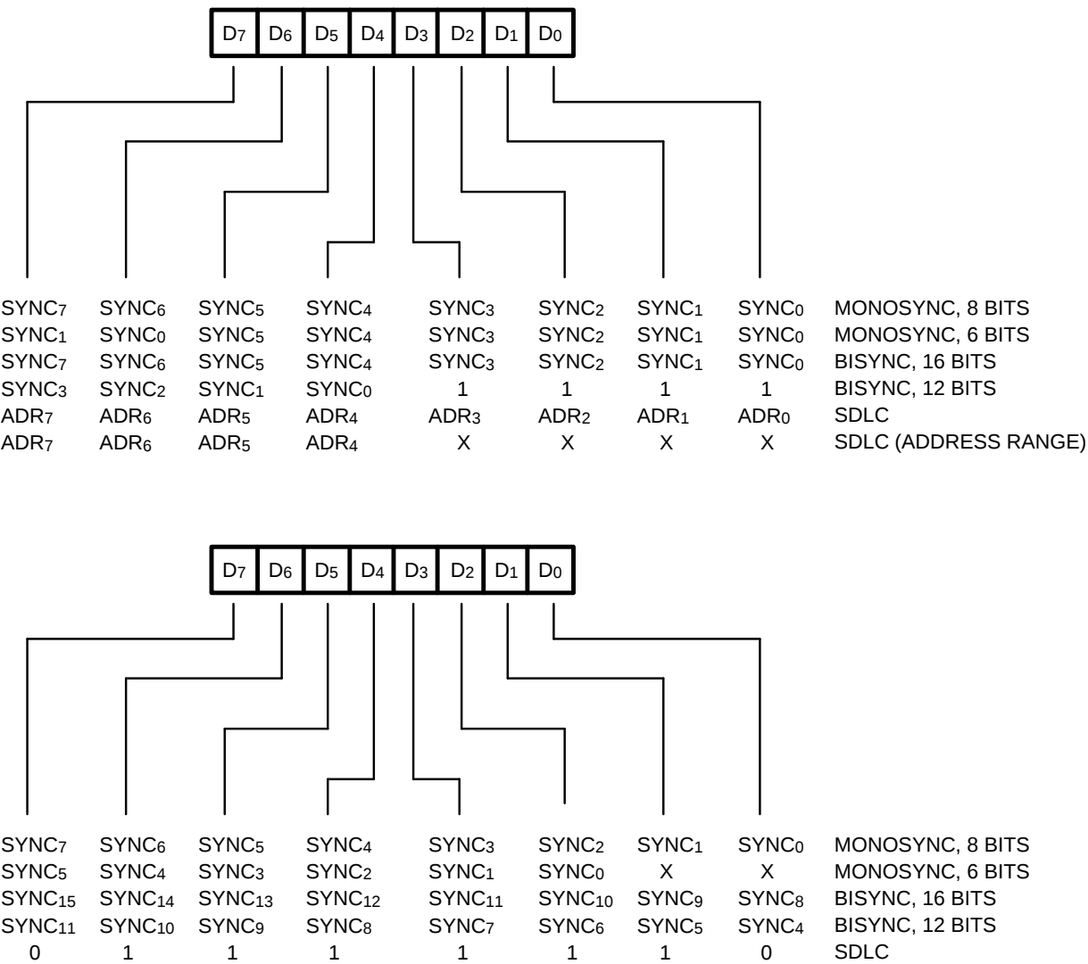
Figure 4-23. SYNC Character Programming
