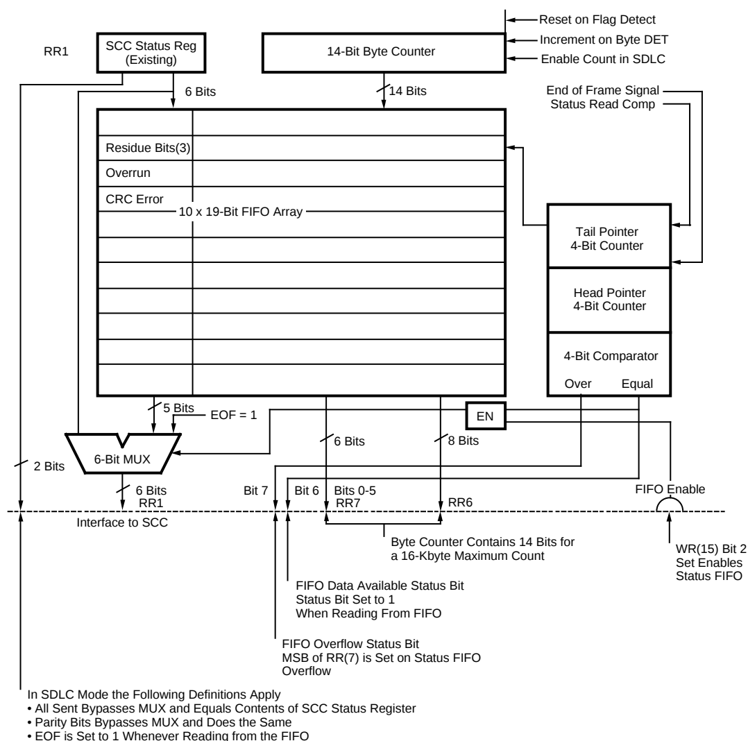
Figure 4–12. 10x19-Bit Frame Status FIFO
