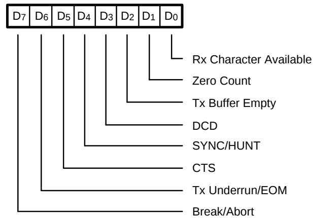
Figure 6–18. Read Register 0
