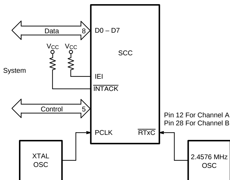
Figure 7–2. SCC Interface
