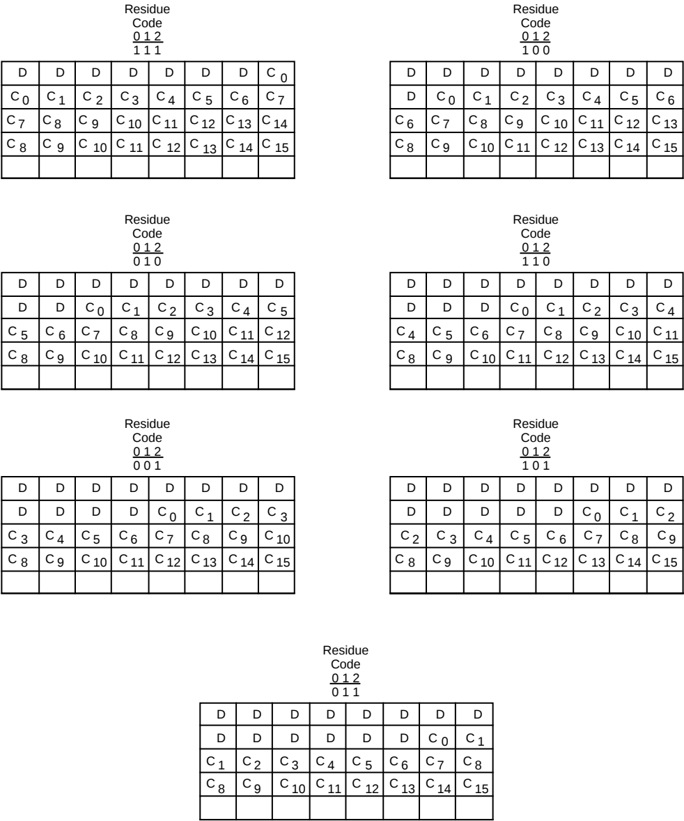
Figure 4-17. Seven Bits/Character
