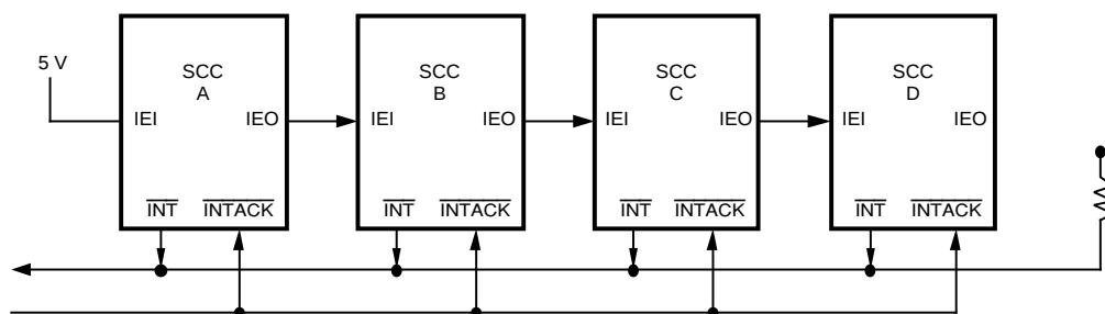
Figure 3-3. External Daisy Chain
