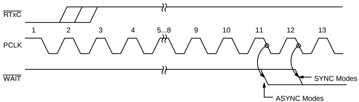
Figure 3–10. \overline{\text{DTR/REQ}} Activation
