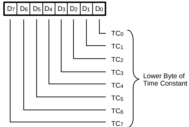
Figure 6–25. Read Register 12
