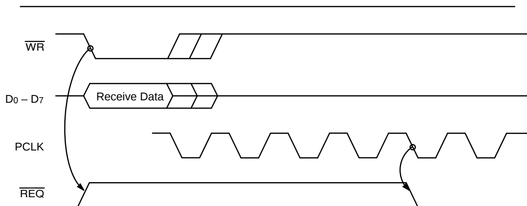
Figure 3–11. \overline{\text{DTR/REQ}} Deactivation
