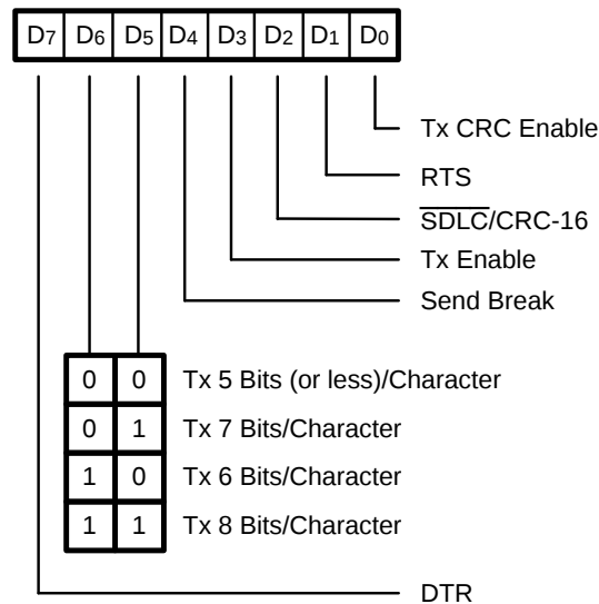
Figure 6–6. Write Register 5
