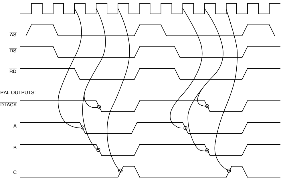
Figure 7–15. PAL Timing
