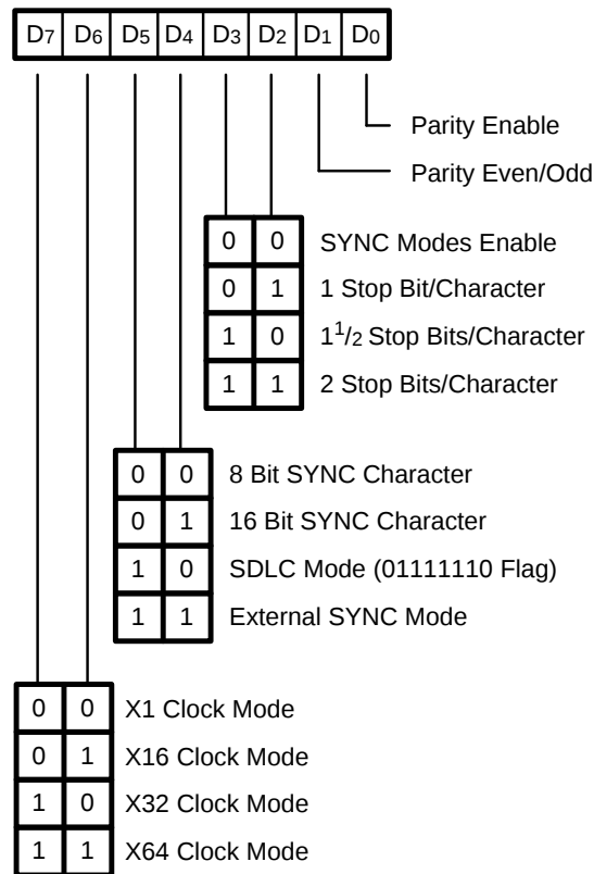
Figure 6–5. Write Register 4
