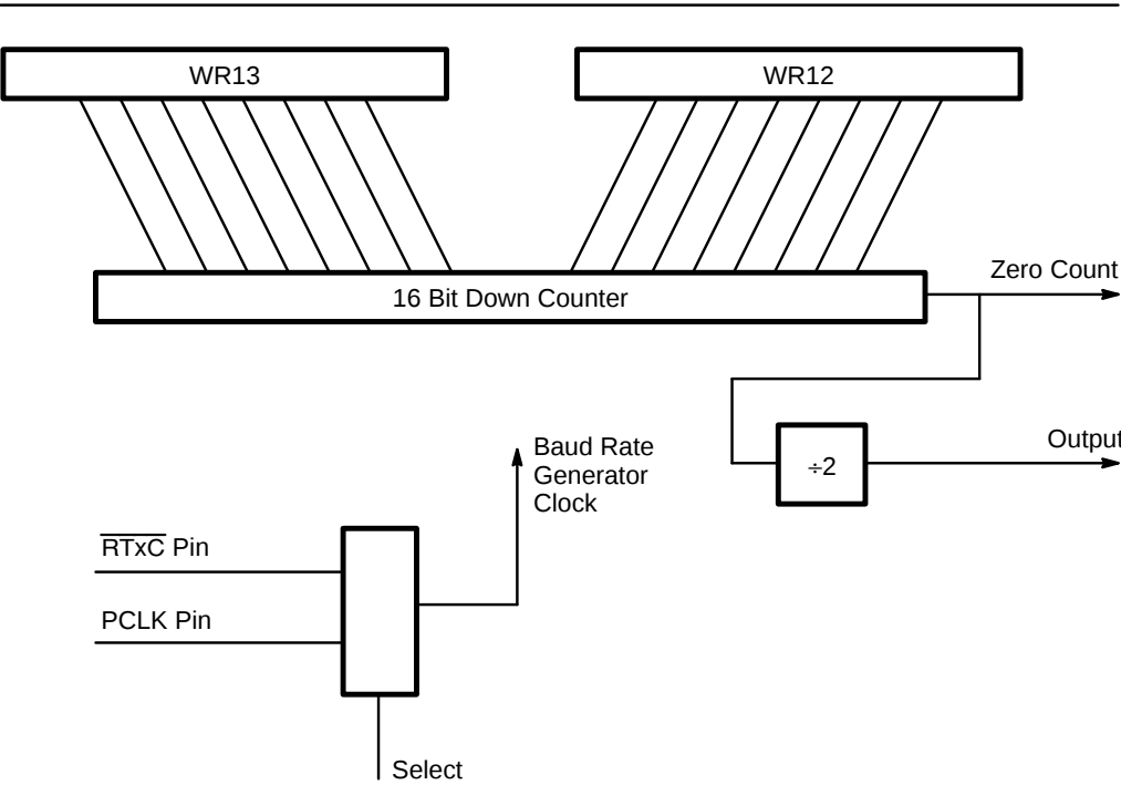
Figure 5–2. Baud Rate Generator
