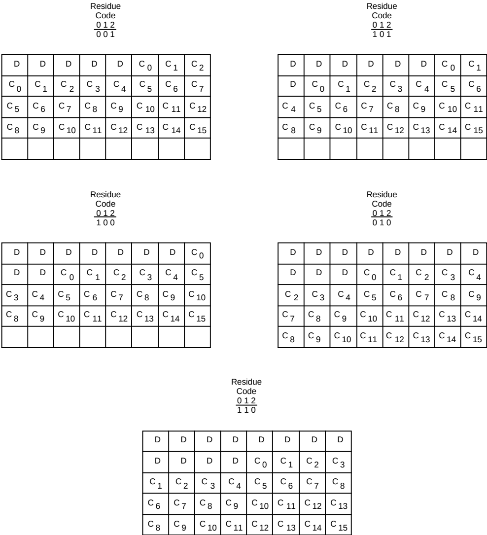
Figure 4–15. Five Bits/Character
