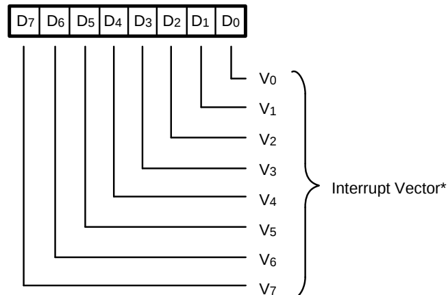
Figure 6–20. Read Register 2
