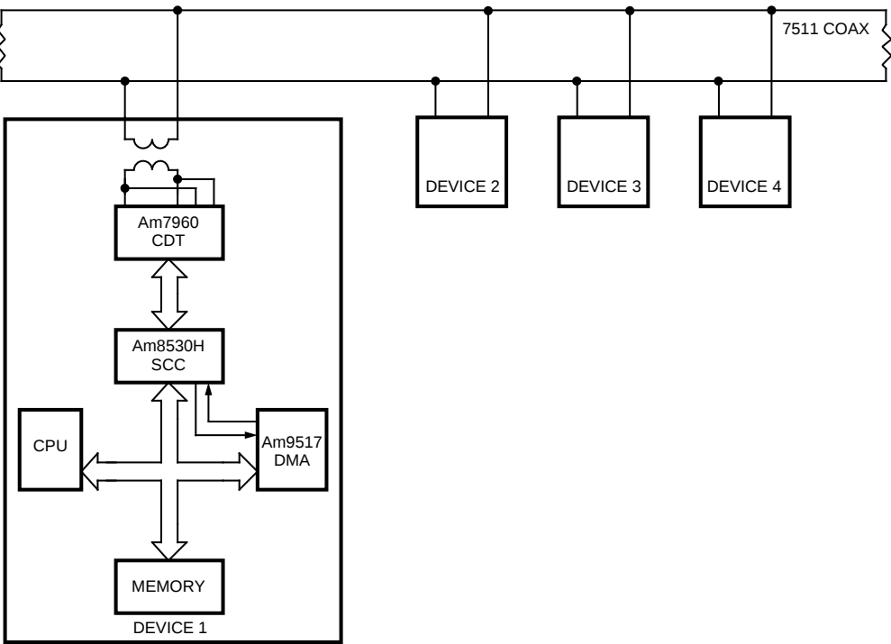
Figure 7-19. Bus Architecture
