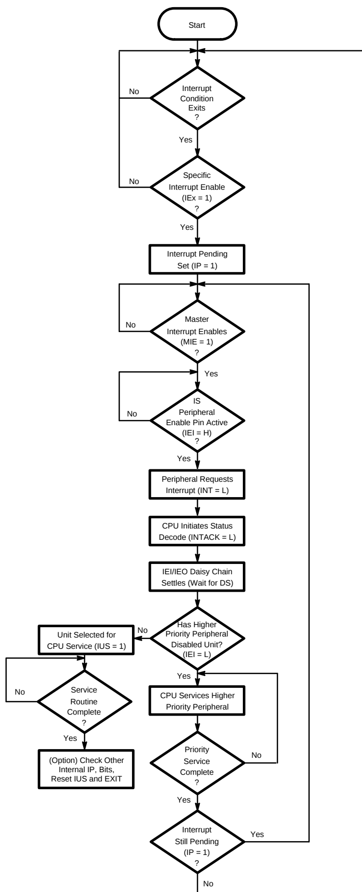
Figure 3–5. Interrupt Protocol
