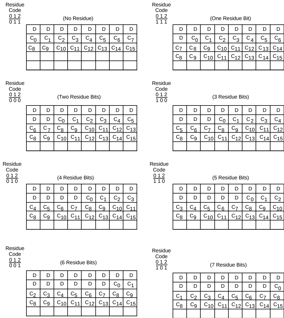
Figure 4–18. Eight Bits/Character
