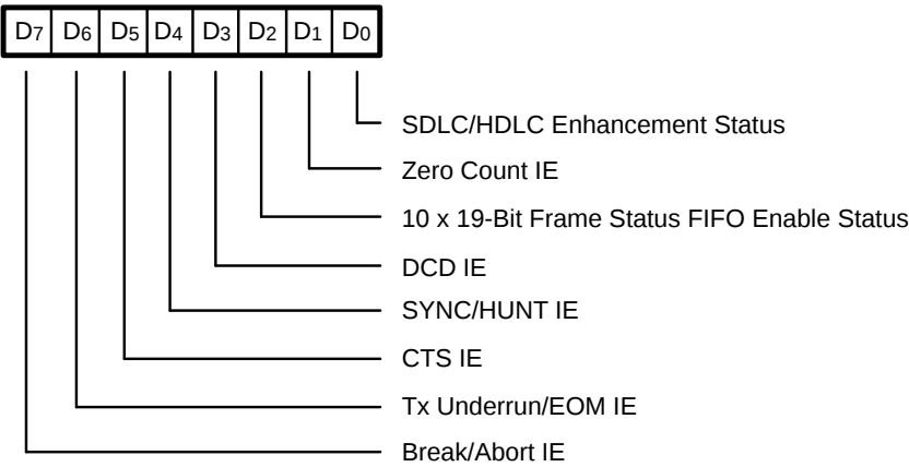
Figure 6–27. Read Register 15
