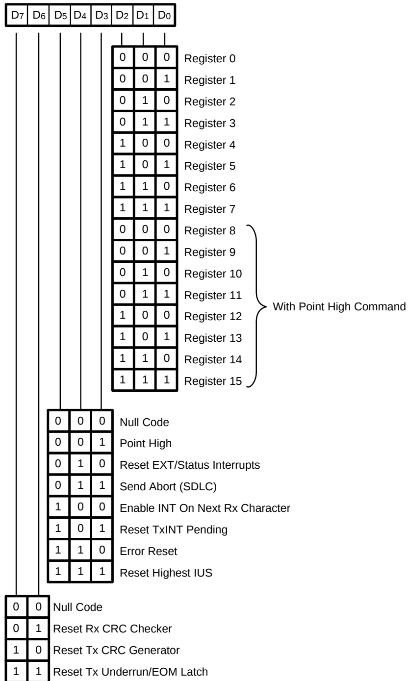
Figure 6–1. Write Register 0
