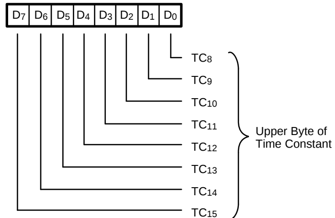
Figure 6–26. Read Register 13
