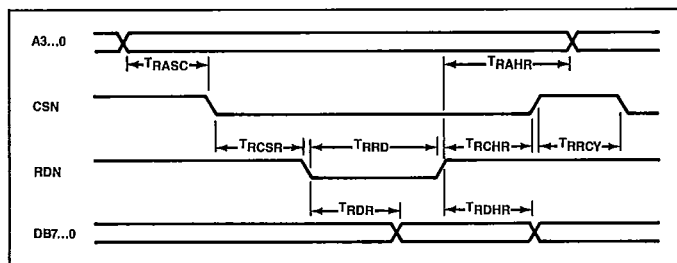
Figure 6. Register Read Operation
