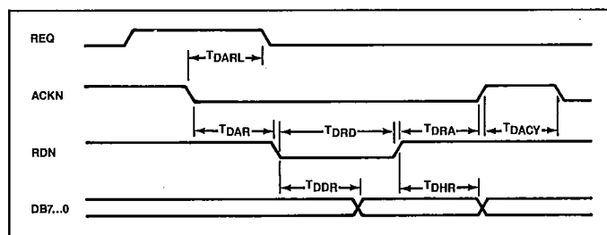
Figure 8. DMA Read Operation
