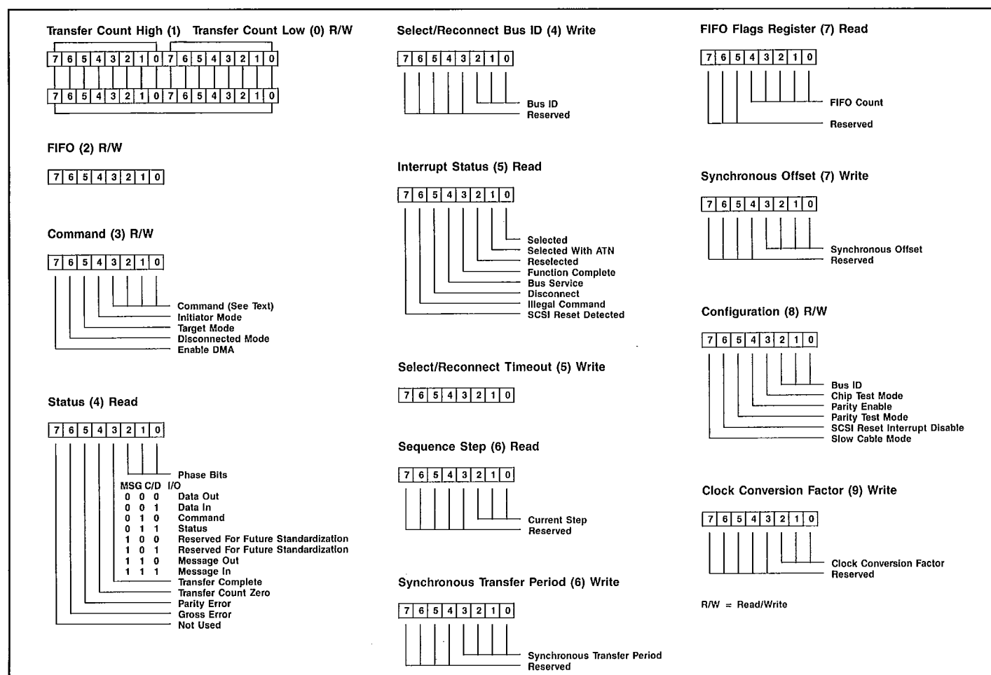
Figure 3. ESP Registers
