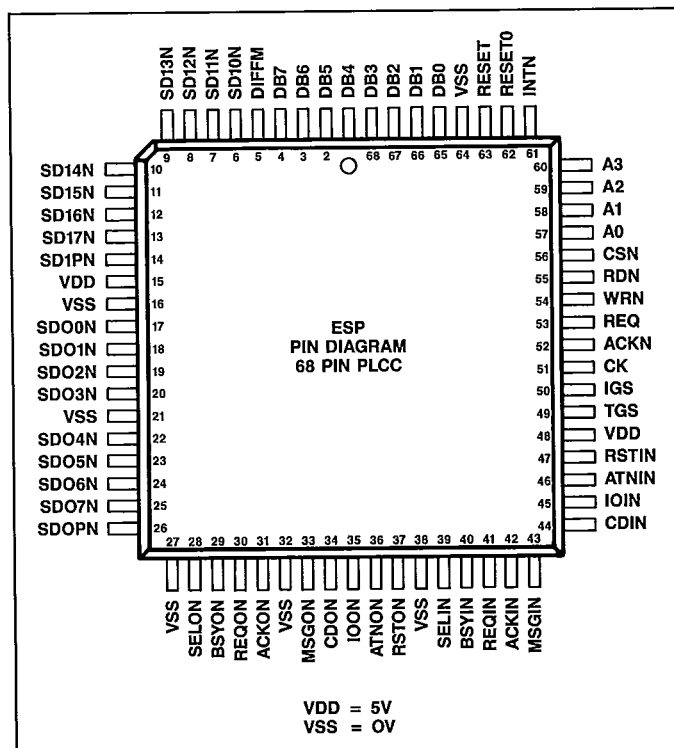
Figure 4. ESP Pinouts
