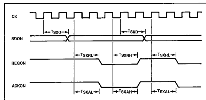
Figure 13. Synchronous Transmit
