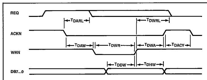
Figure 7. DMA Write Operation
