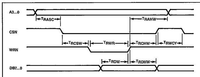
Figure 5. Register Write Operation
