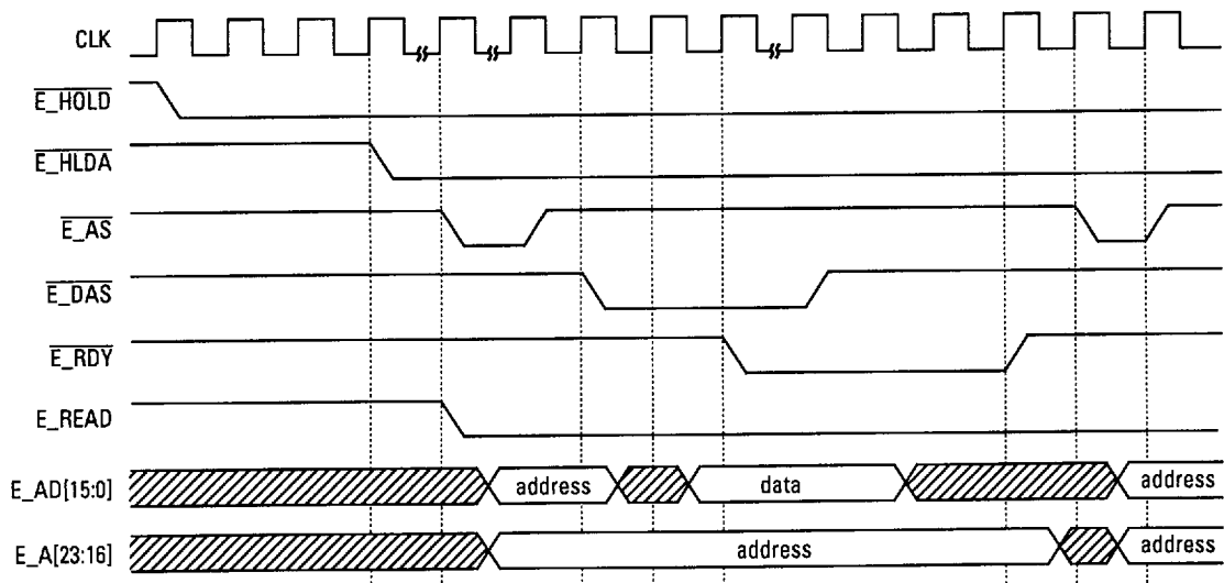
Figure 5.2 E-Channel DMA Write
