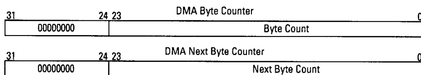
Figure 2.3 DMA Byte and Next Byte Counters
