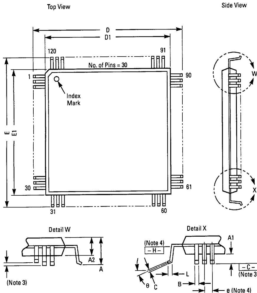
Figure 7.14 120-Pin PQFP Mechanical Drawing
