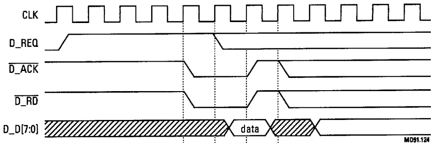
Figure 4.6 DMA Write with FASTER = 1 , SLOW = 1
