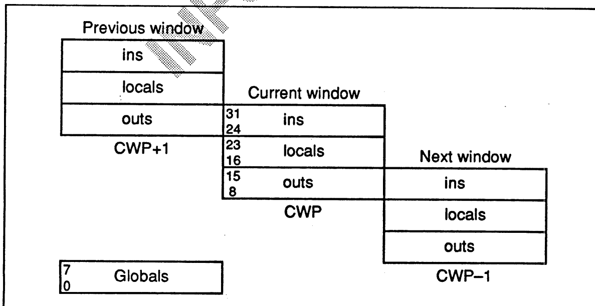
Figure 3 — Register Windowing in the BIT SPARC
