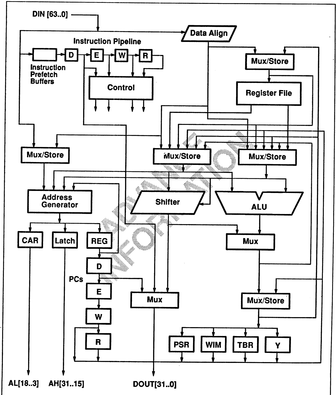
Figure 2 — BIT SPARC Integer Unit Block Diagram
