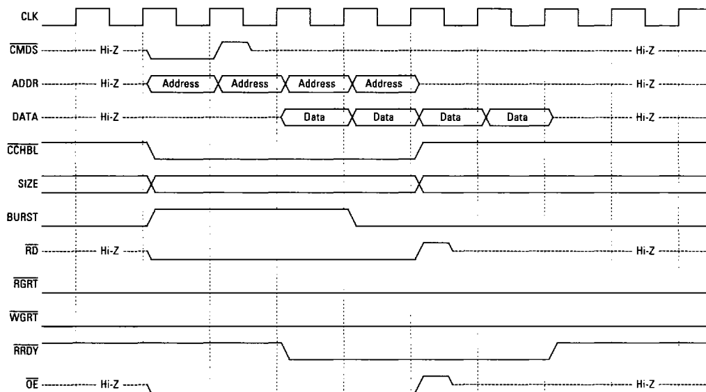
Figure 15. VBus Burst Read Hit
