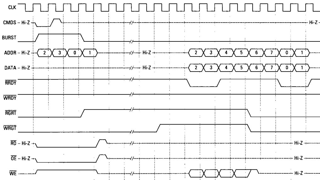
Figure 16. VBus Burst Read Miss
