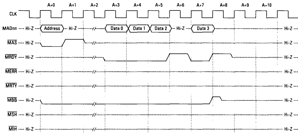
Figure 6. MBus Burst Read
