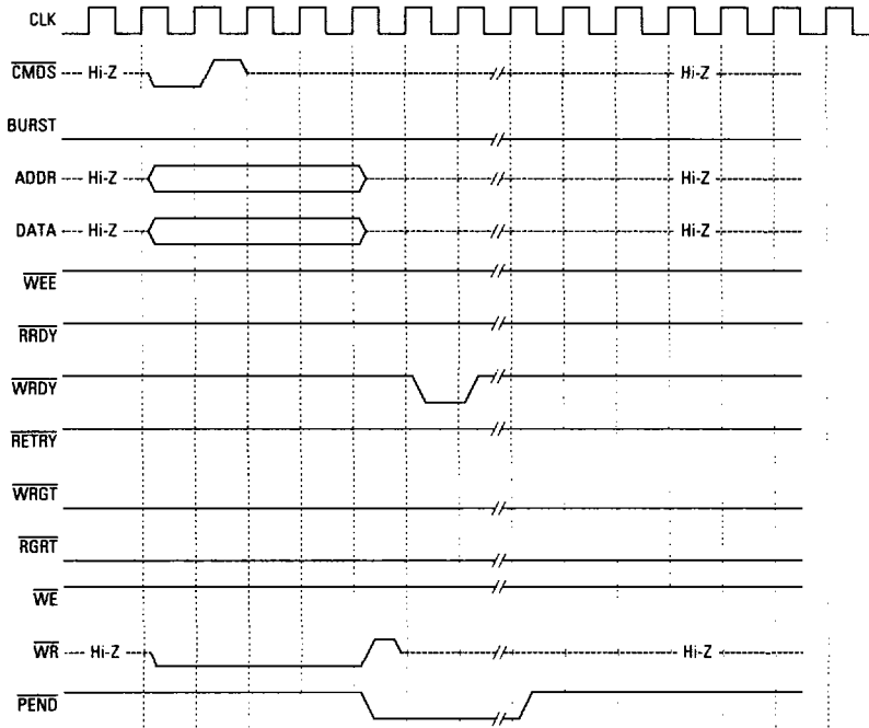
Figure 12. VBus Cache Disabled/Non-Cacheable Single Write
