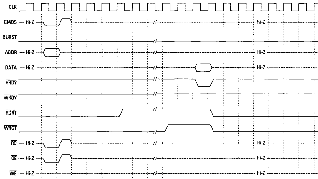
Figure 11. VBus Cache Disabled/Non-Cacheable Single Read
