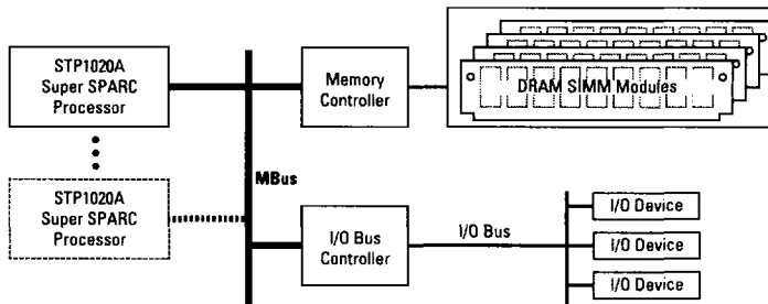
Figure 1. Typical STP1020A Uniprocessor / Multiprocessor MBus System
