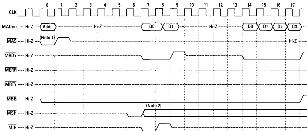
Figure 7. MBUS Coherent Read of Shared Data
