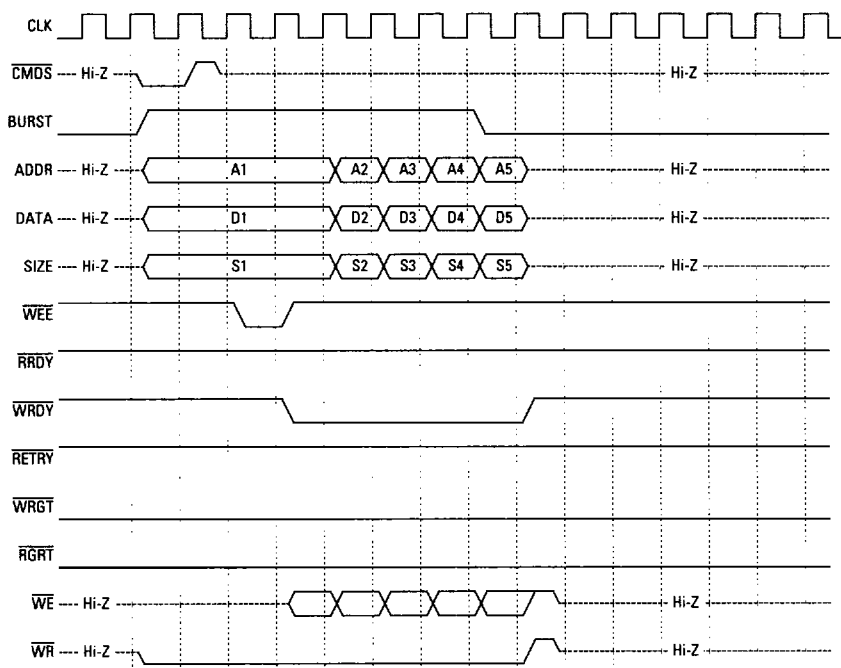
Figure 18. VBus Cacheable Burst Write Hit
