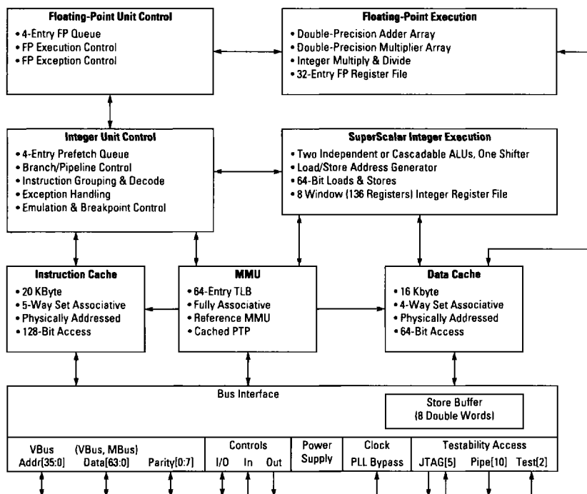
Figure 3. STP1020A SuperSPARC Functional Block Diagram
