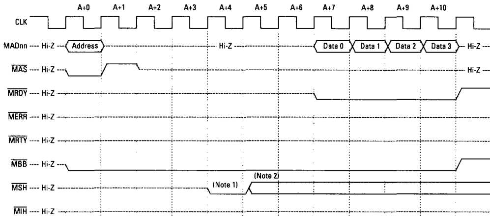
Figure 7. MBUS Coherent Read of Shared Data
