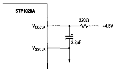
Figure 20. Typical Phase Lock Loop (PLL) Filter Circuit
