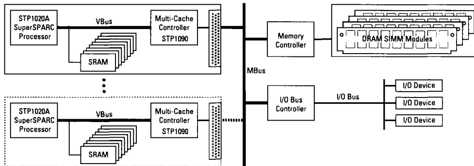
Figure 2. Typical STP1020A Uniprocessor / Multiprocessor System with External Cache Controller
