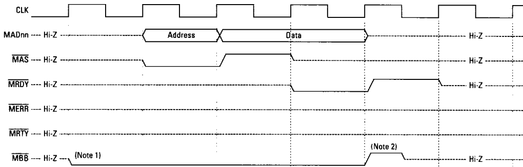
Figure 5. MBus Single Write
