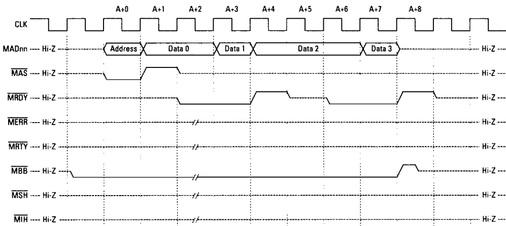
Figure 10. MBus Coherent Write and Invalidate
