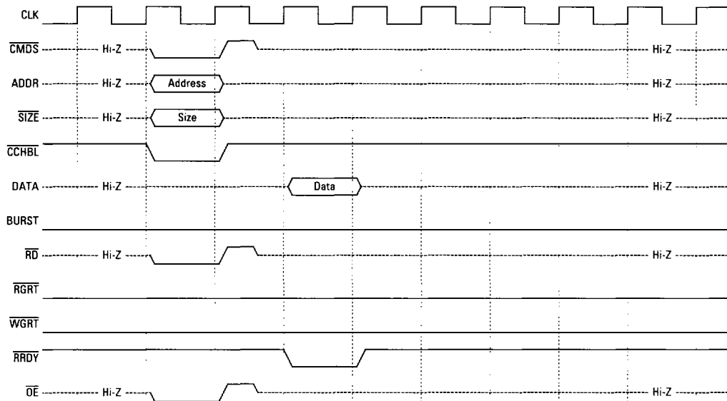
Figure 13. VBus Cacheable Single Read Hit
