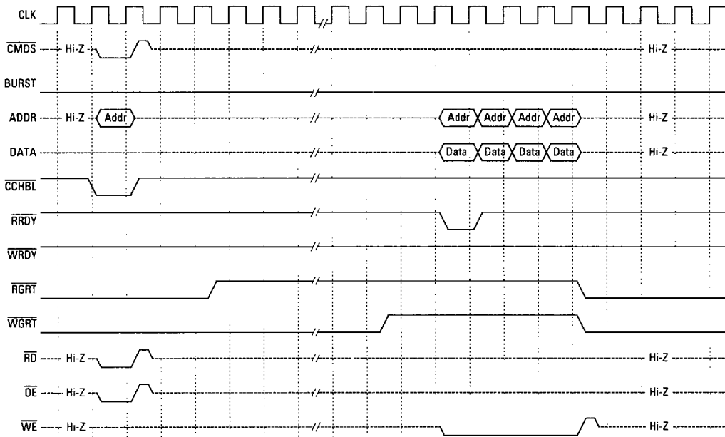
Figure 14. VBus Cacheable Single Read Miss
