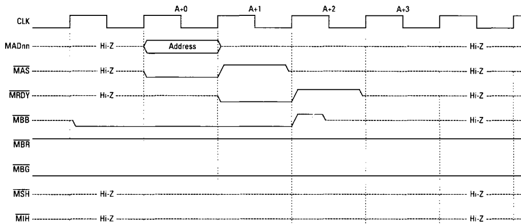
Figure 9. MBus Coherent Invalidate
