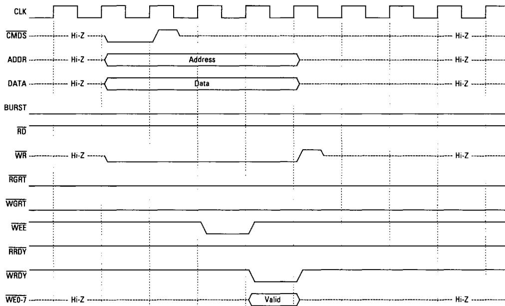
Figure 17. VBus Cacheable Single Write Hit
