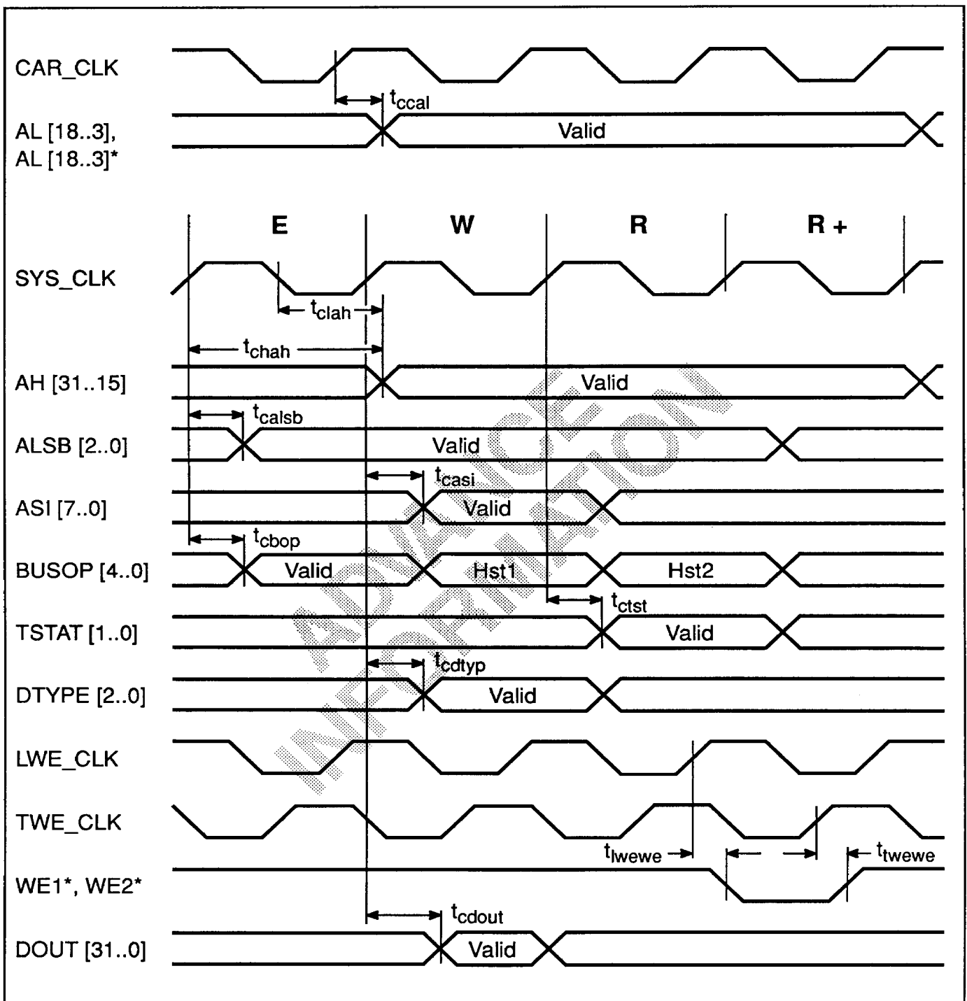
Figure 11 — Store Timing with No MHOLD
