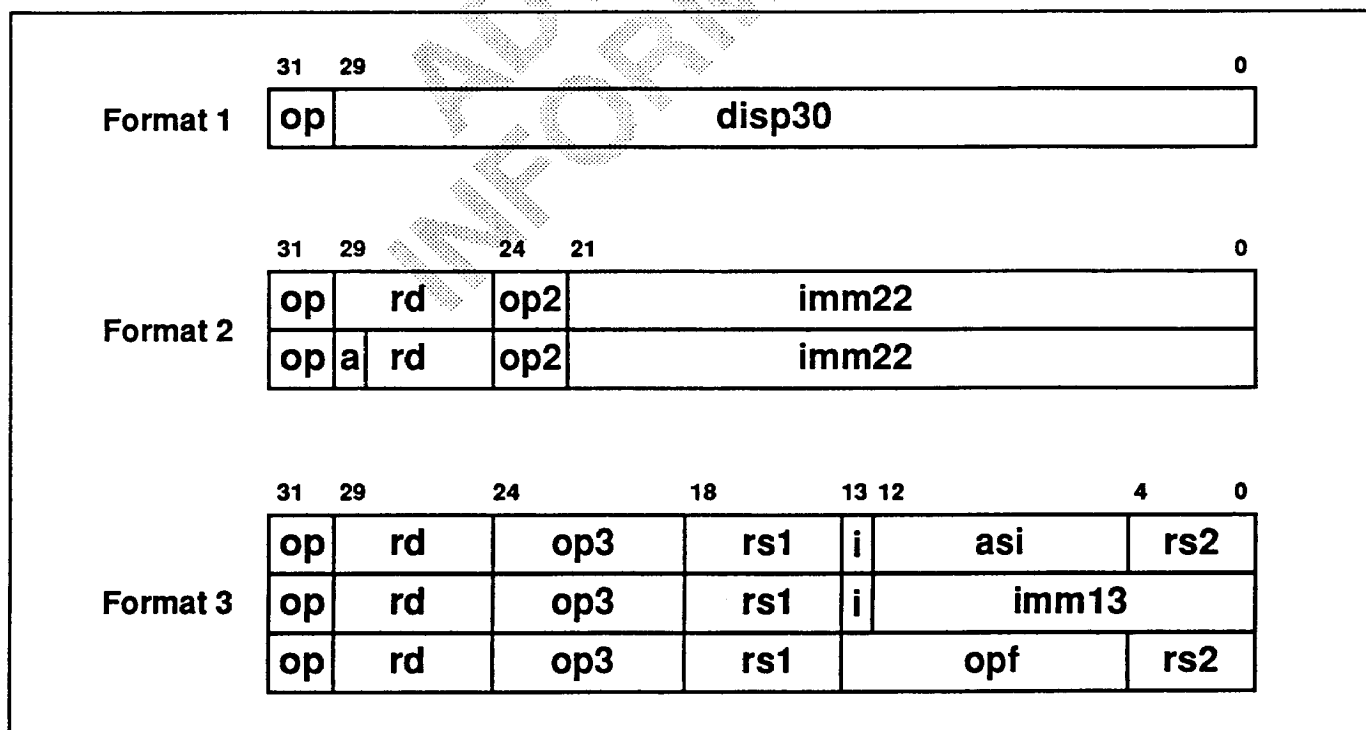
Figure 6 — BIT SPARC Instruction Formats
