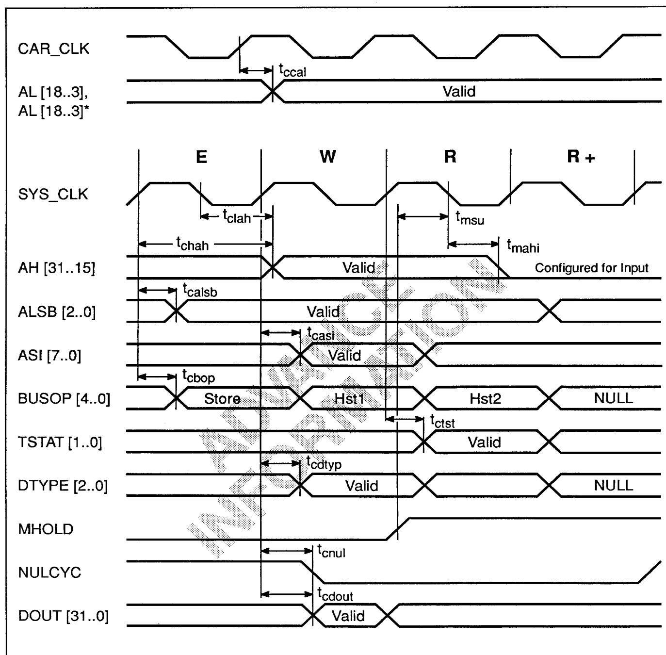
Figure 12 — Store Timing with MHOLD
