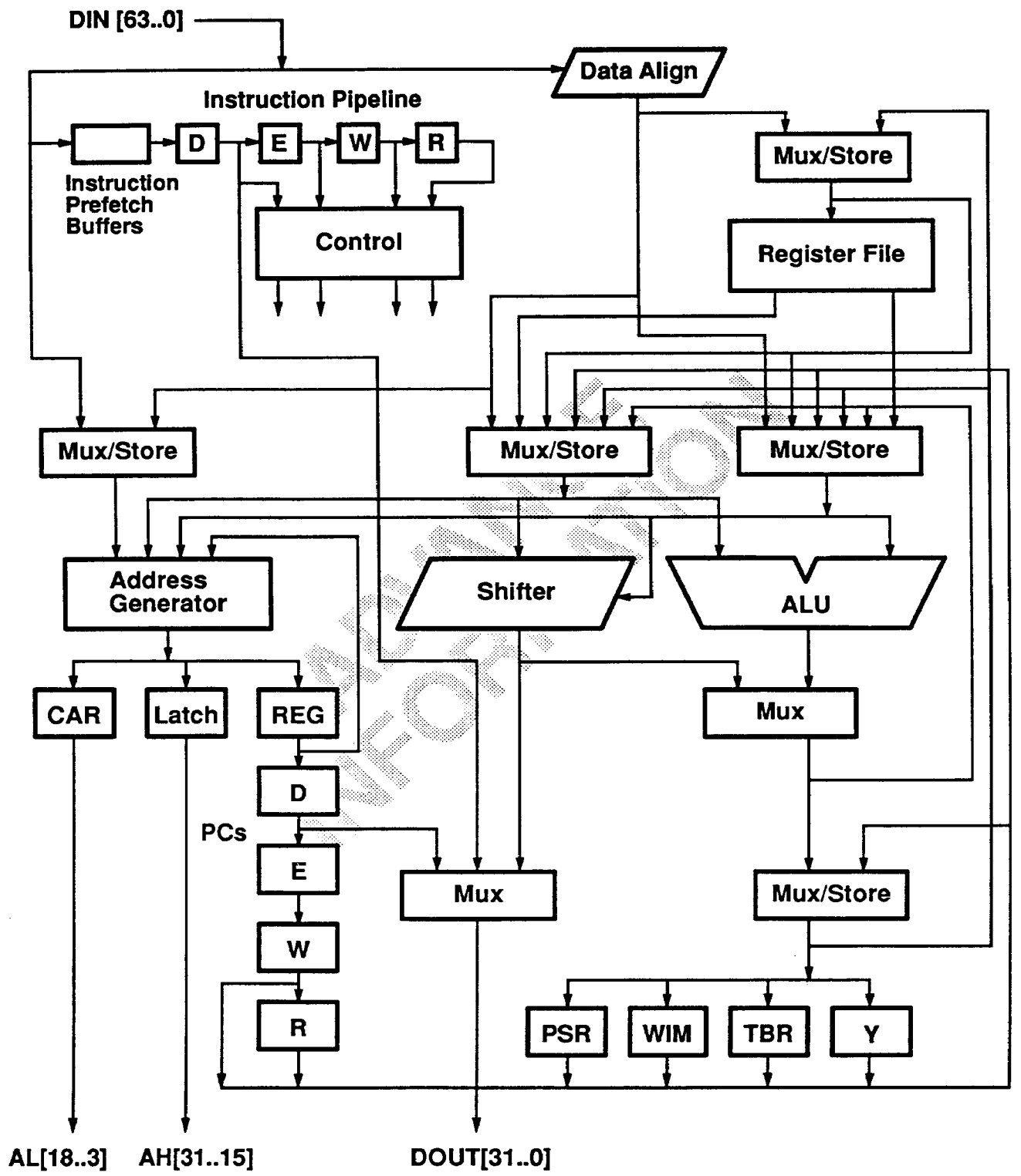
Figure 1 — BIT SPARC Integer Unit Block Diagram
