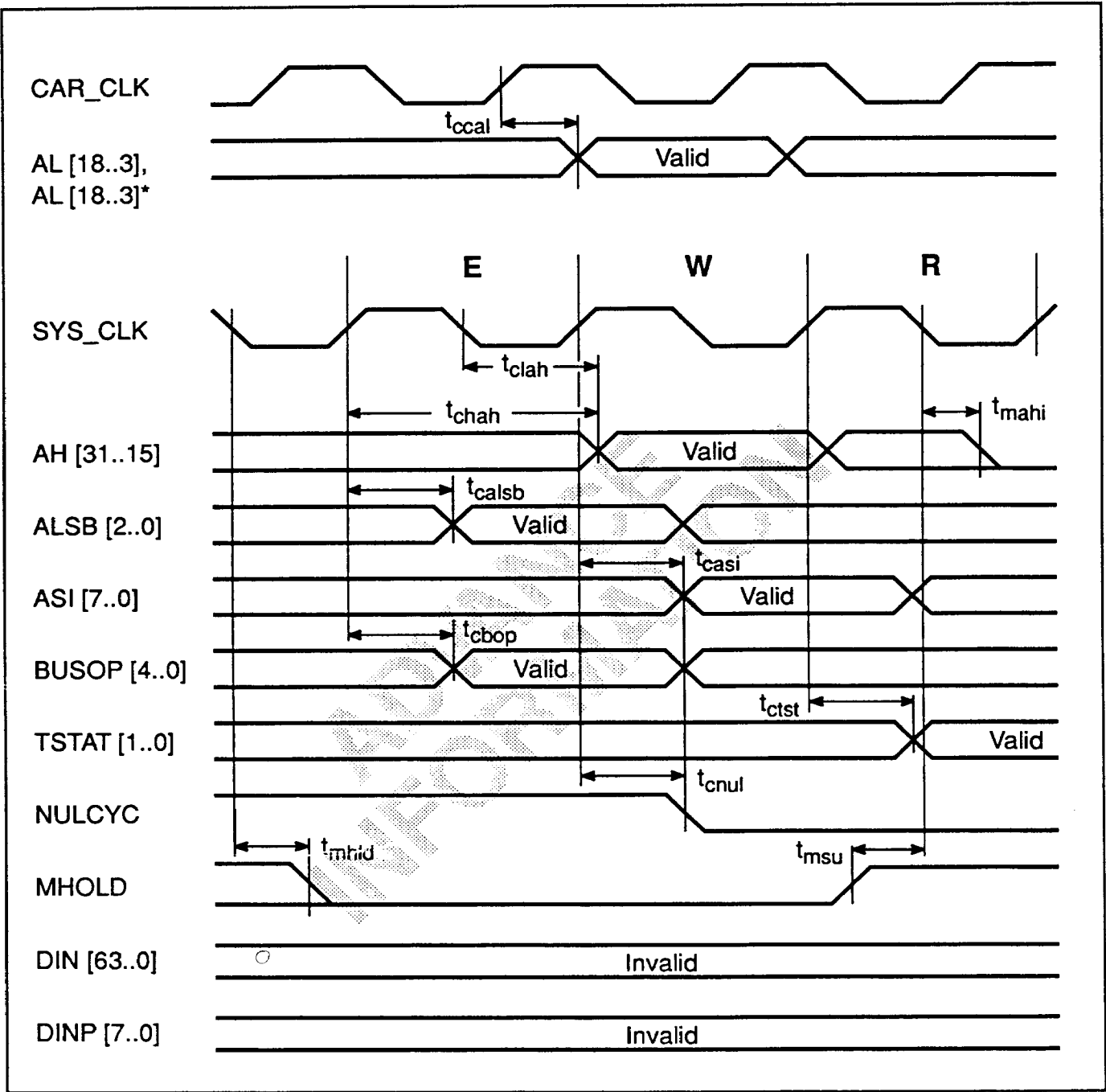
Figure 10 — Load/Fetch Timing with MHOLD
