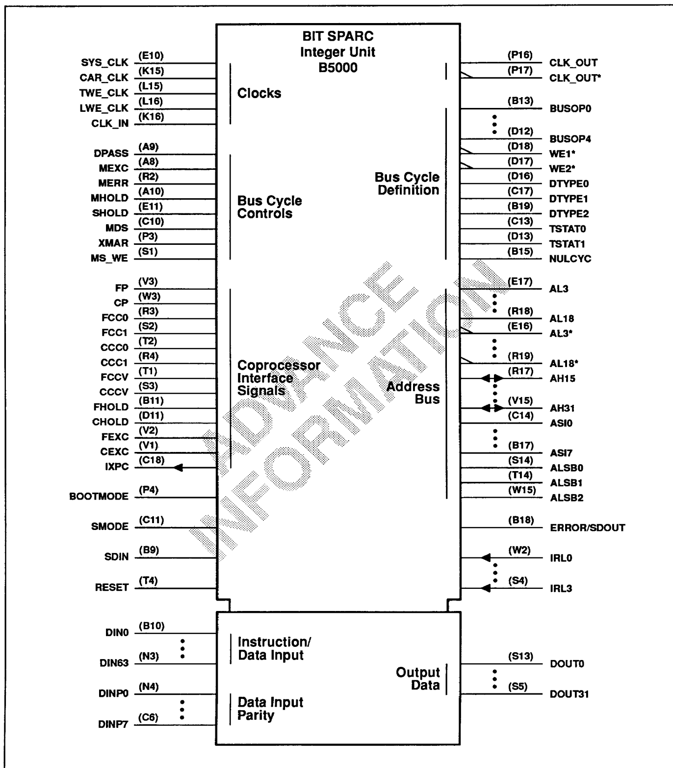
Figure 7 — BIT SPARC Integer Unit Pin Assignments
