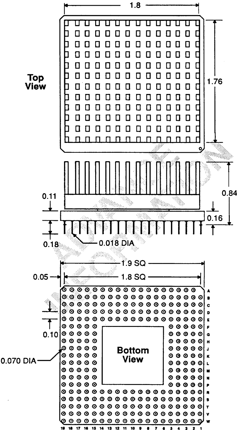
Figure 14 — B5000 Package Dimensions
