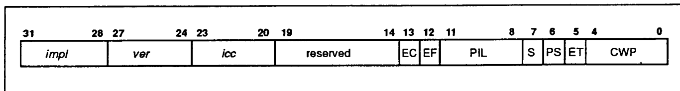
Figure 3 — BIT SPARC Processor State Register (PSR)
