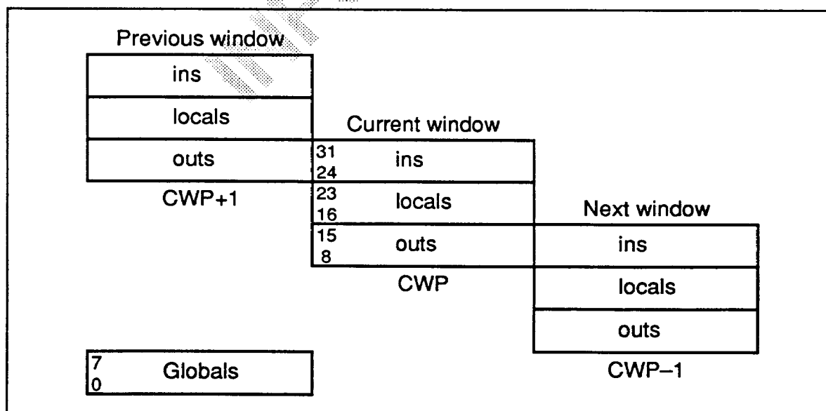
Figure 2 — Register Windowing in the BIT SPARC
