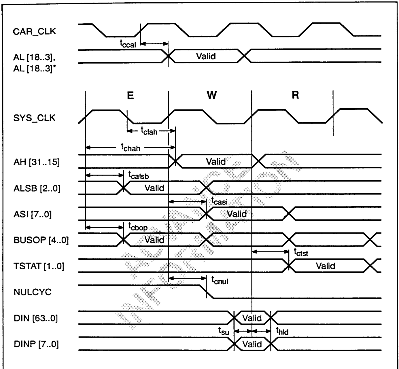
Figure 9 — Load/Fetch Timing with No MHOLD
