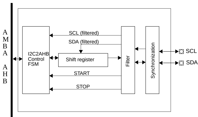
Figure 177. Block diagram, optional APB interface not shown
