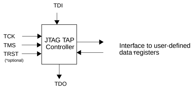
Figure 288. TAP controller block diagram
