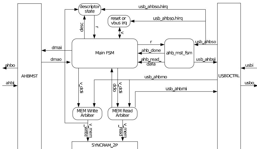
Figure 290. Block diagram of the internal structure of the GRUSBDC. Blocks with rounded corners are implemented as VHDL procedures while squares represent VHDL entities.
