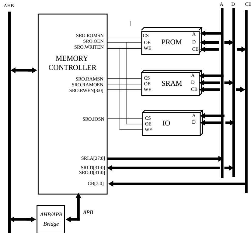
Figure 274. 8/32-bit PROM/SRAM/IO controller
