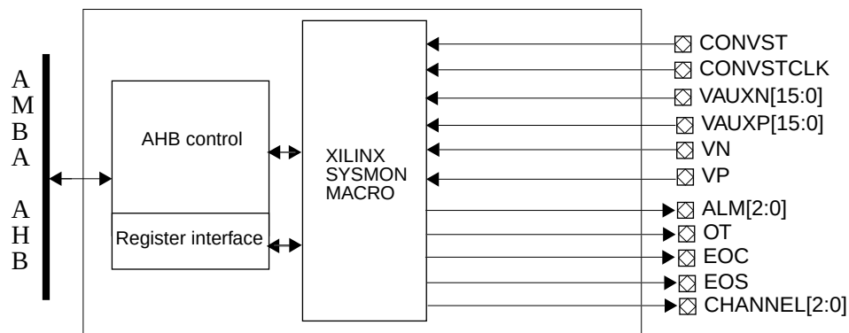
Figure 171. Block diagram
