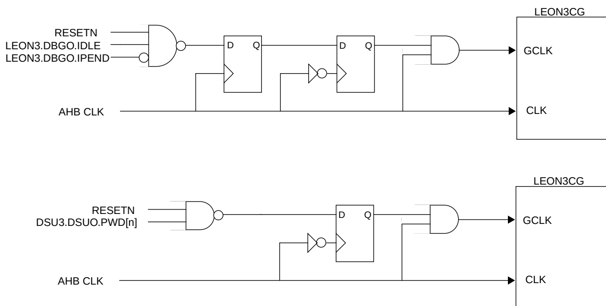
Figure 198. Examples of LEON3 clock gating
