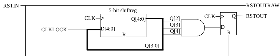
Figure 266. Reset generator with VHDL generic syncrst set to 0 and scan test disabled
