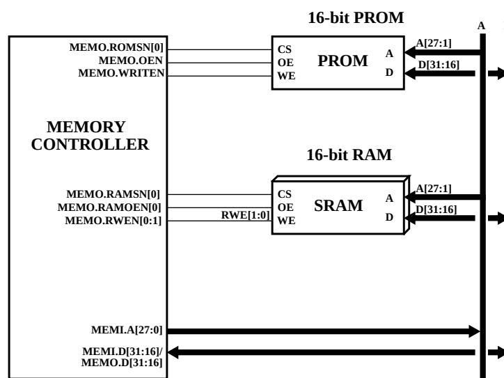
Figure 232. 16-bit memory interface example
