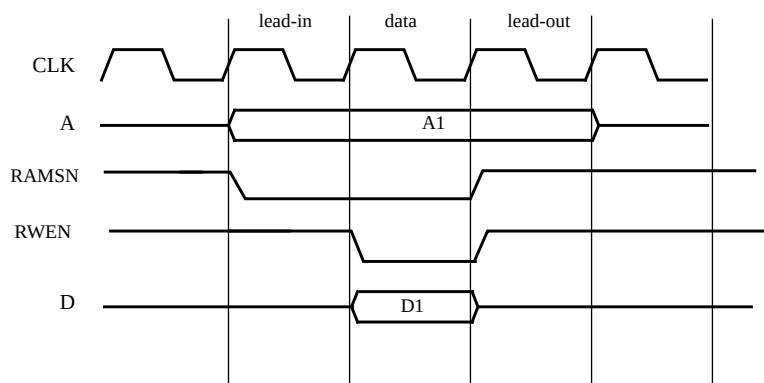
Figure 276. 32-bit PROM/SRAM/IO write cycle
