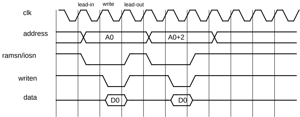
Figure 283. 32-bit PROM/IO write cycle in 16-bit mode
