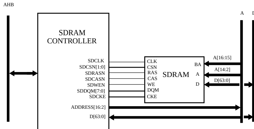
Figure 268. SDRAM Memory controller connected to AMBA bus and SDRAM
