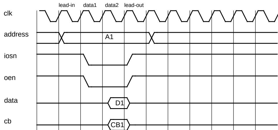
Figure 227. I/O read cycle (0-waitstates)
