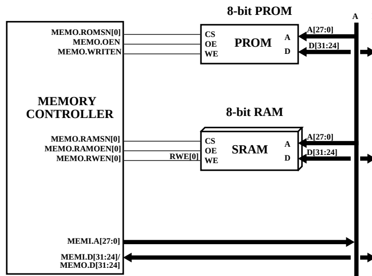
Figure 231. 8-bit memory interface example
