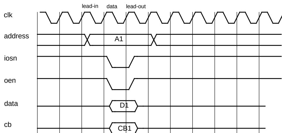
Figure 228. I/O write cycle (0-waitstates)
