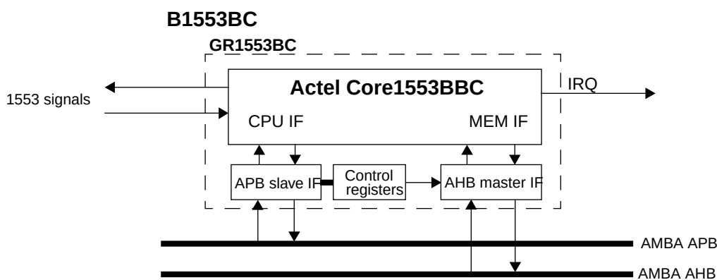
Figure 30. Block diagram
