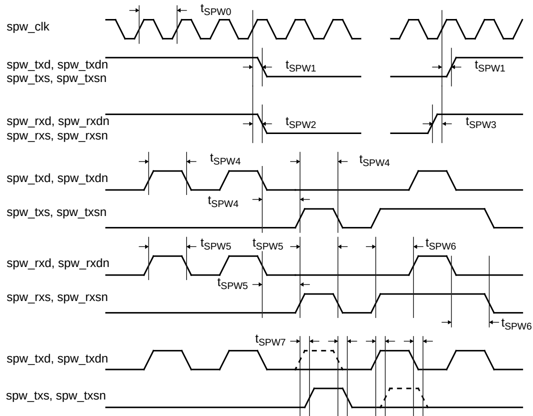
Figure 164. Timing waveforms
