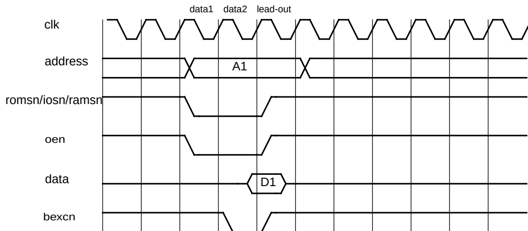
Figure 235. Read cycle with BEXCN.
