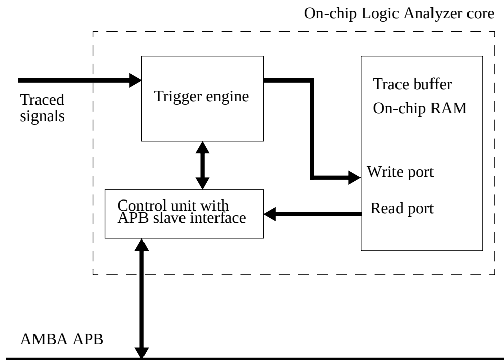
Figure 213. On-chip Logic Analyzer block diagram
