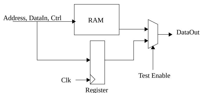
Figure 285. Scan test support
