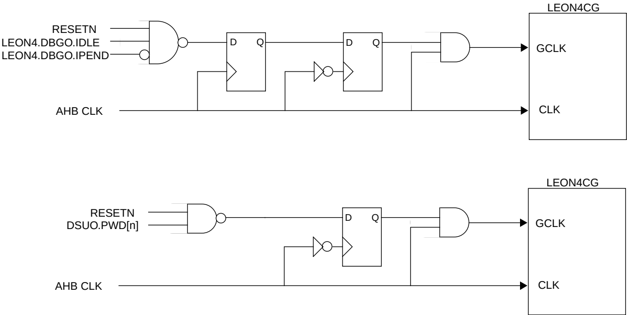
Figure 212. Examples of LEON4 clock gating
