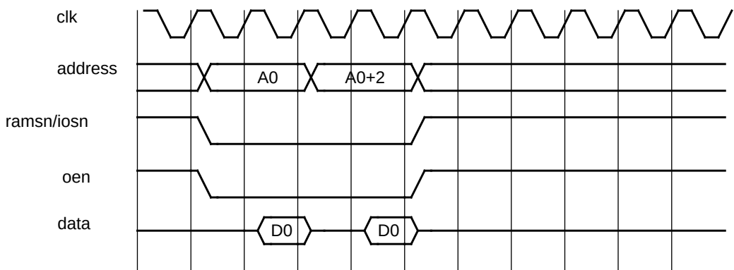
Figure 282. 32-bit PROM/IO read cycle in 16-bit mode
