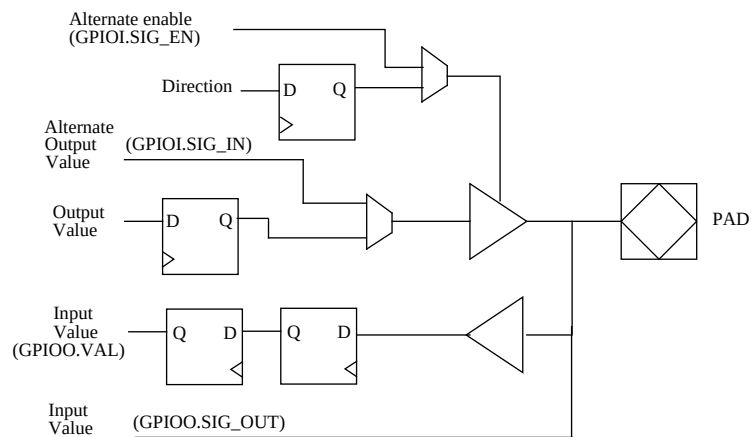
Figure 155. General Purpose I/O Port diagram
