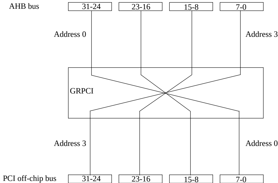
Figure 251. GRPCI byte twisting
