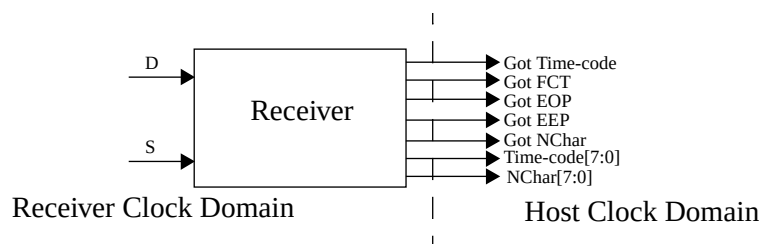
Figure 162. Schematic of the link interface receiver.
