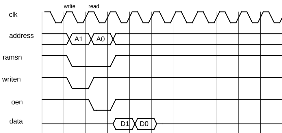
Figure 279. 32-bit SSRAM write cycle
