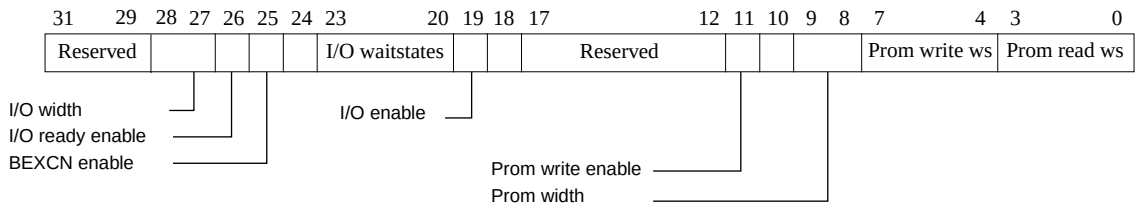
Figure 284. Memory configuration register
