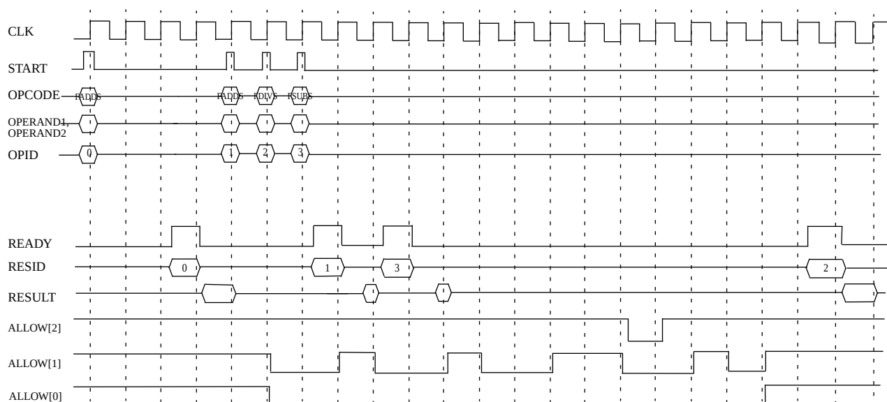
Figure 154. Signal timing
