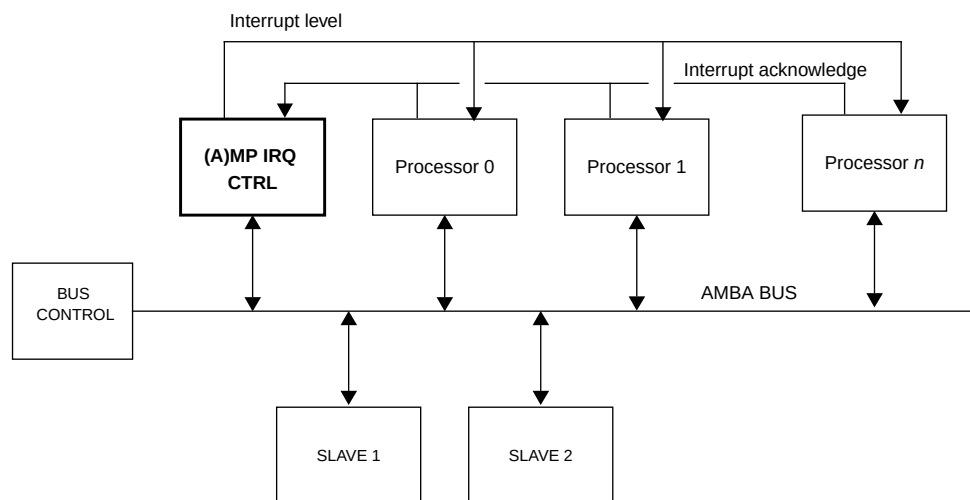
Figure 185. LEON multiprocessor system with Multiprocessor Interrupt controller
