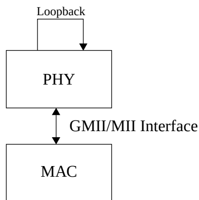
Figure 264. Block diagram of the PHY simulation model connected to a MAC.
