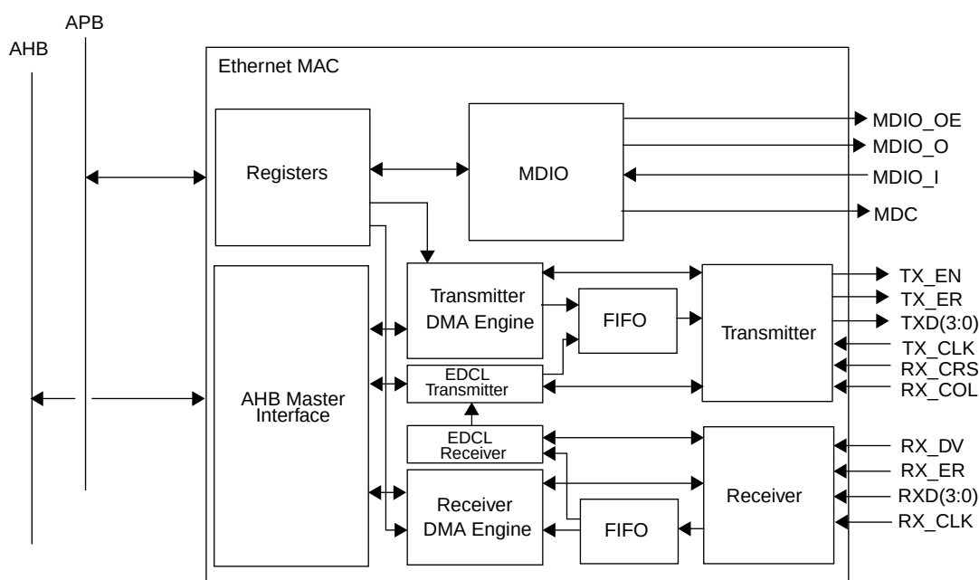
Figure 143. Block diagram of the internal structure of the GRETH.
