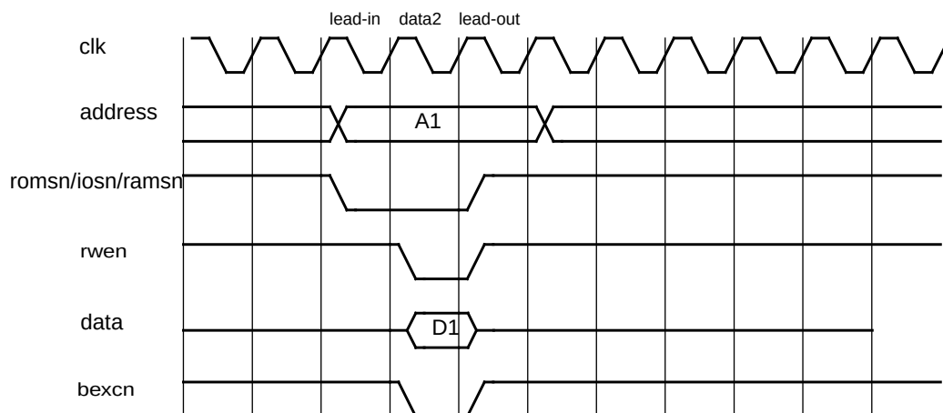
Figure 236. Write cycle with BEXCN. Chip-select (iosn) is not asserted in lead-in cycle for io-accesses.
