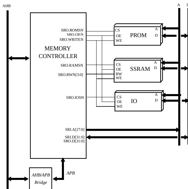
Figure 277. 32-bit SSRAM/PROM/IO controller
