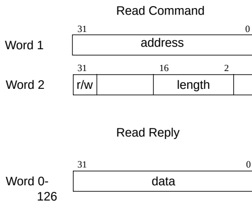
Figure 293. Layout of USB DCL read commands and replies.
