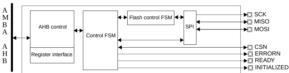
Figure 273. Block diagram
