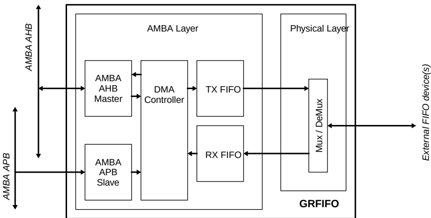
Figure 145. Block diagram
