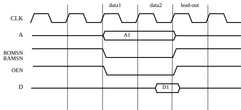
Figure 275. 32-bit PROM/SRAM/IO read cycle
