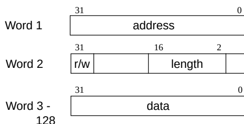
Figure 292. Layout of USB DCL write commands.
