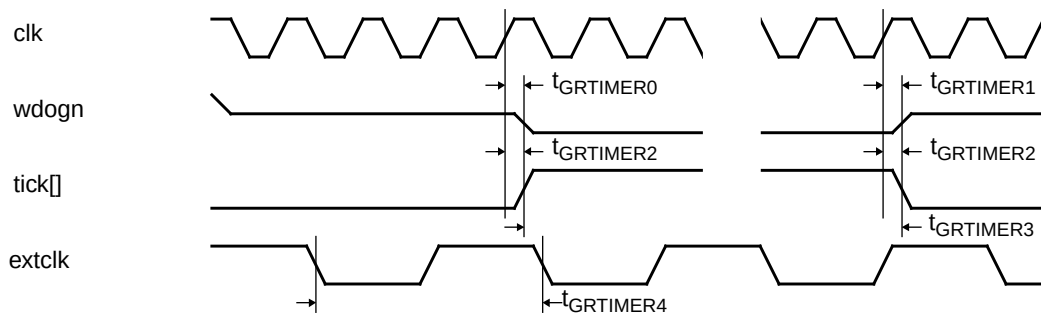
Figure 138. Timing waveforms
