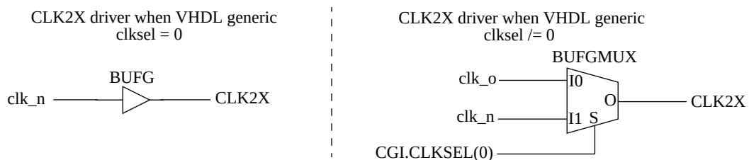
Figure 58. Virtex 2/4 selection of CLK2X clock when VHDL generic clk2xen is non-zero
