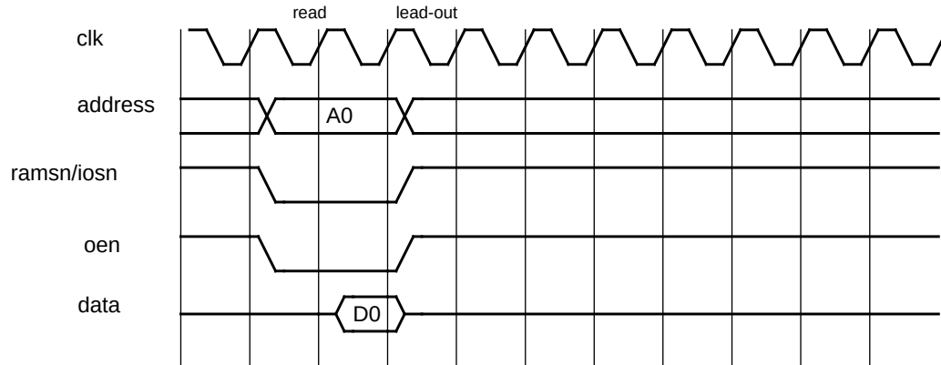
Figure 280. 32-bit PROM/I/O read cycle
