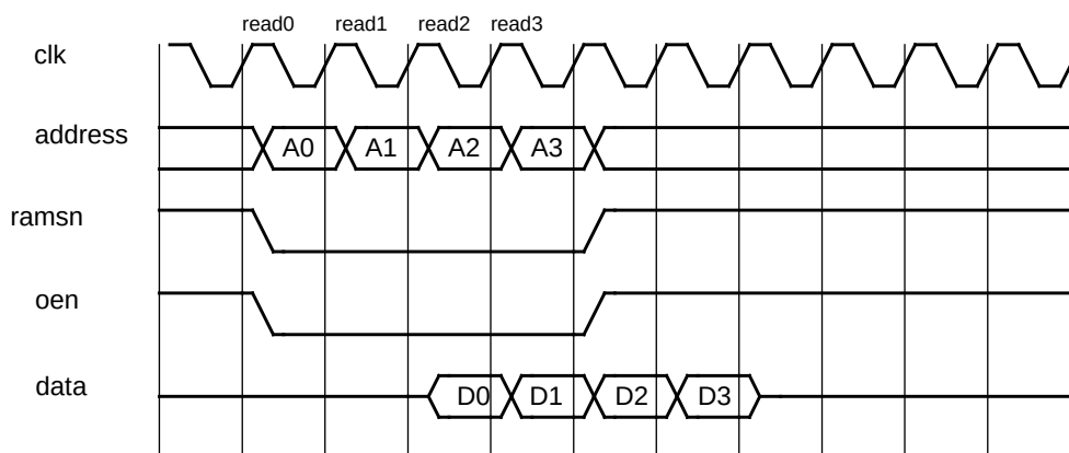
Figure 278. 32-bit SSRAM read cycle
