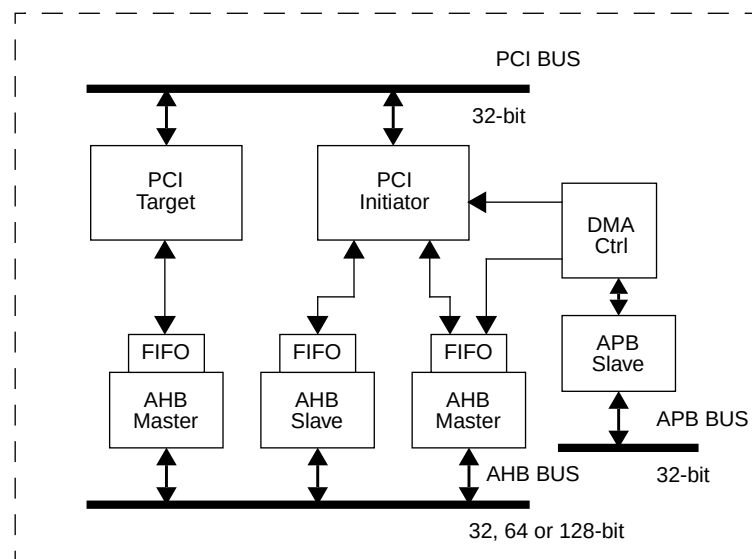
Figure 255. Block diagram
