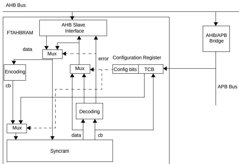
Figure 82. Block diagram
