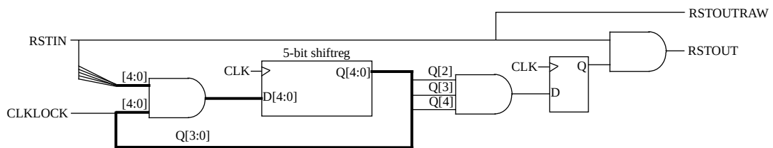
Figure 265. Reset generator with VHDL generic syncrst set to 1
