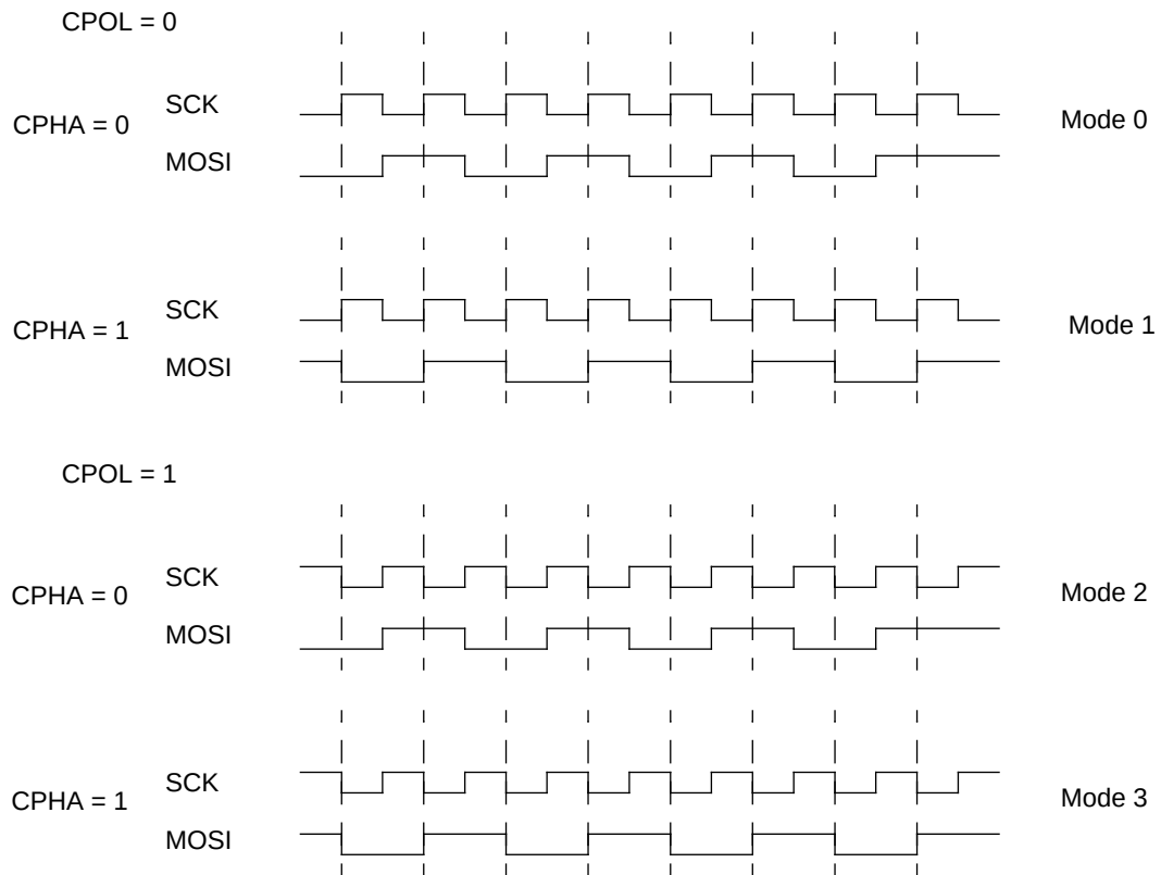
Figure 270. SPI transfer of byte 0x55 in all modes
