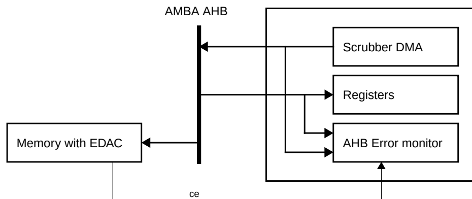
Figure 237. Memory scrubber block diagram
