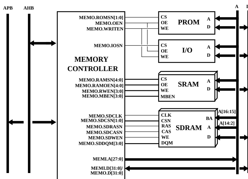
Figure 221. Memory controller connected to AMBA bus and different types of memory devices
