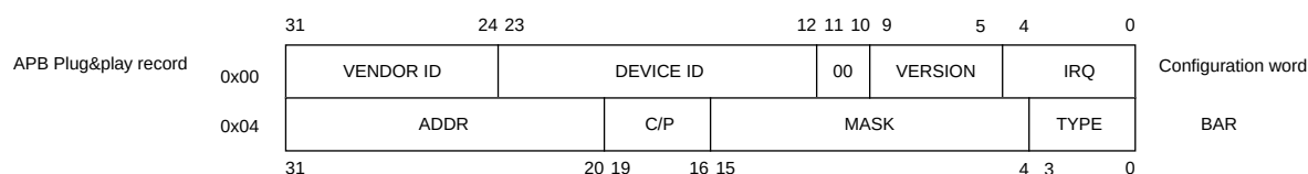
Figure 15. APB plug&play information
