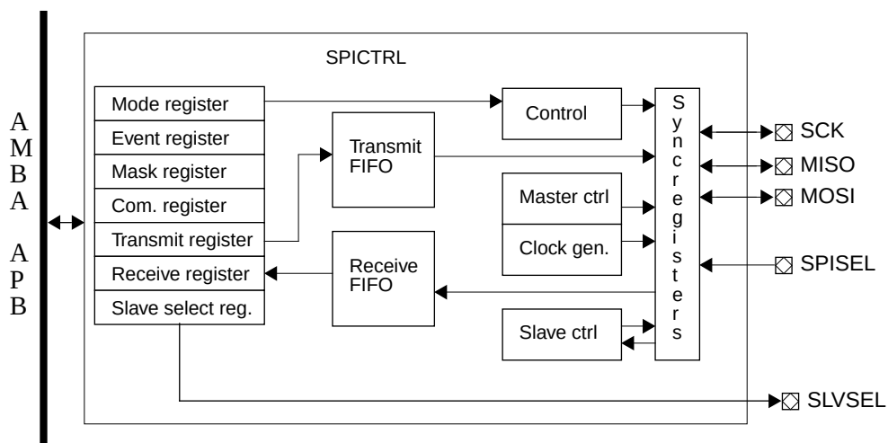
Figure 271. Block diagram
