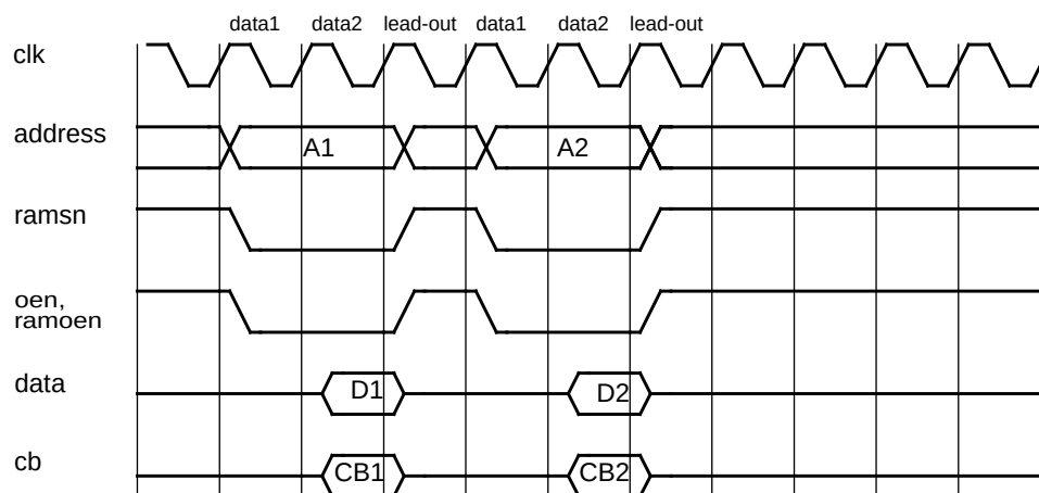
Figure 229. SRAM non-consecutive read cycles.
