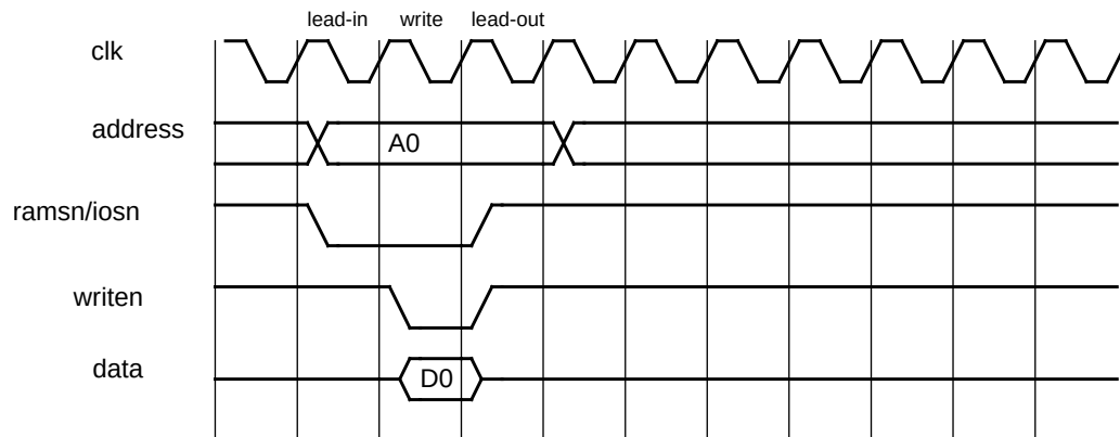
Figure 281. 32-bit PROM/I/O write cycle
