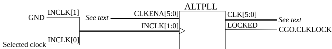
Figure 44. Altera Cyclone III ALTPLL
