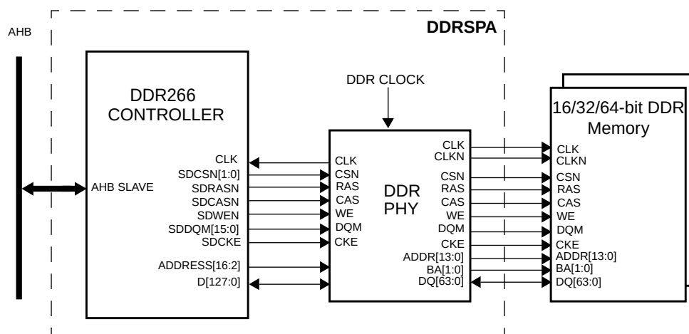
Figure 68. DDRSPA Memory controller connected to AMBA bus and DDR SDRAM
