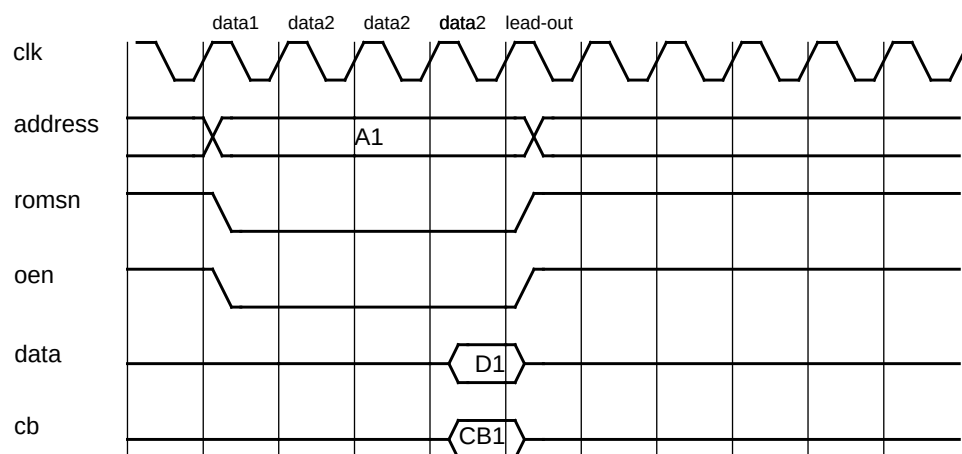
Figure 224. Prom read access with two waitstates.
