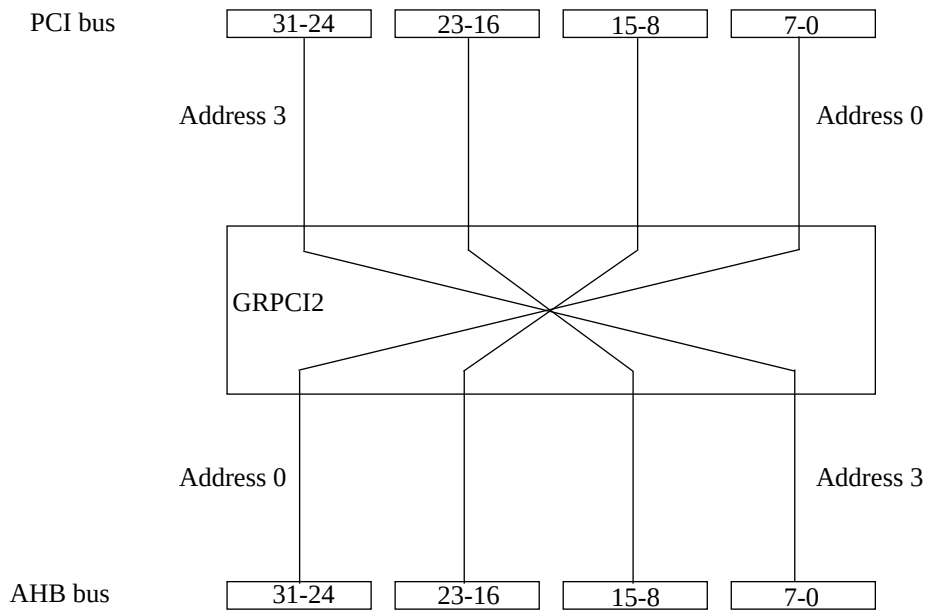
Figure 256. GRPCI2 byte twisting
