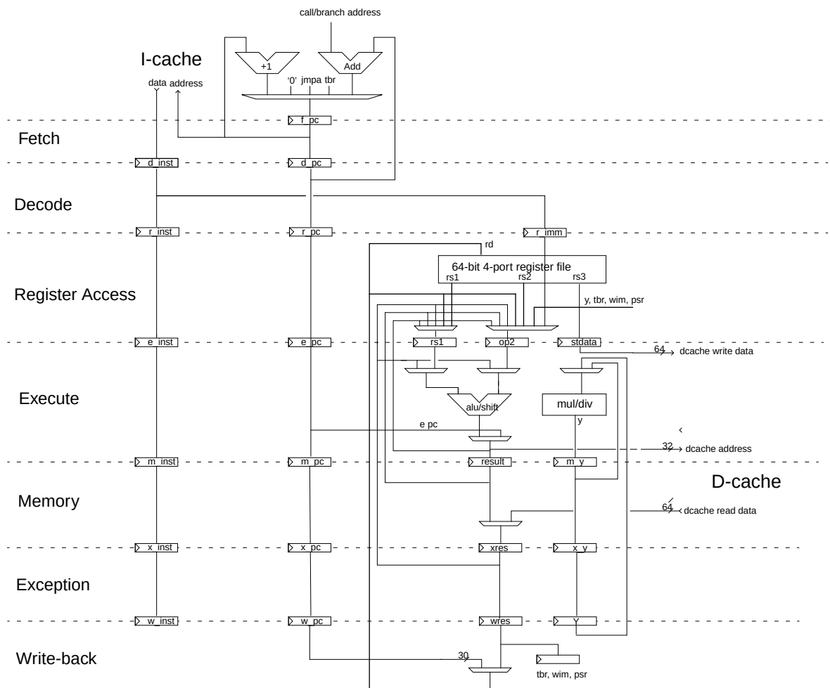
Figure 204. LEON4 integer unit datapath diagram
