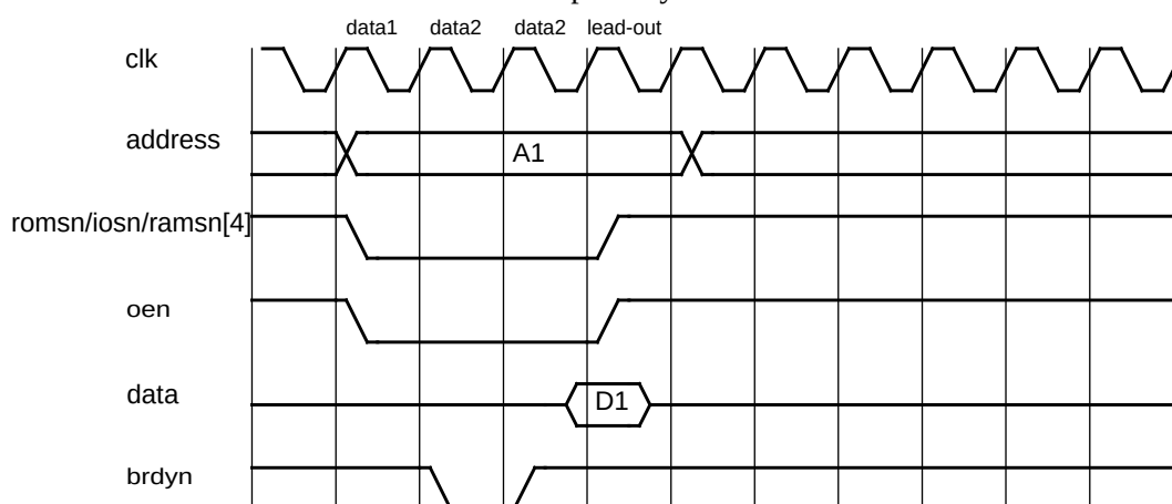
Figure 233. READ cycle with one extra data2 cycle added with BRDYN (synchronous sampling). Lead-out cycle is only applicable for I/O accesses.
