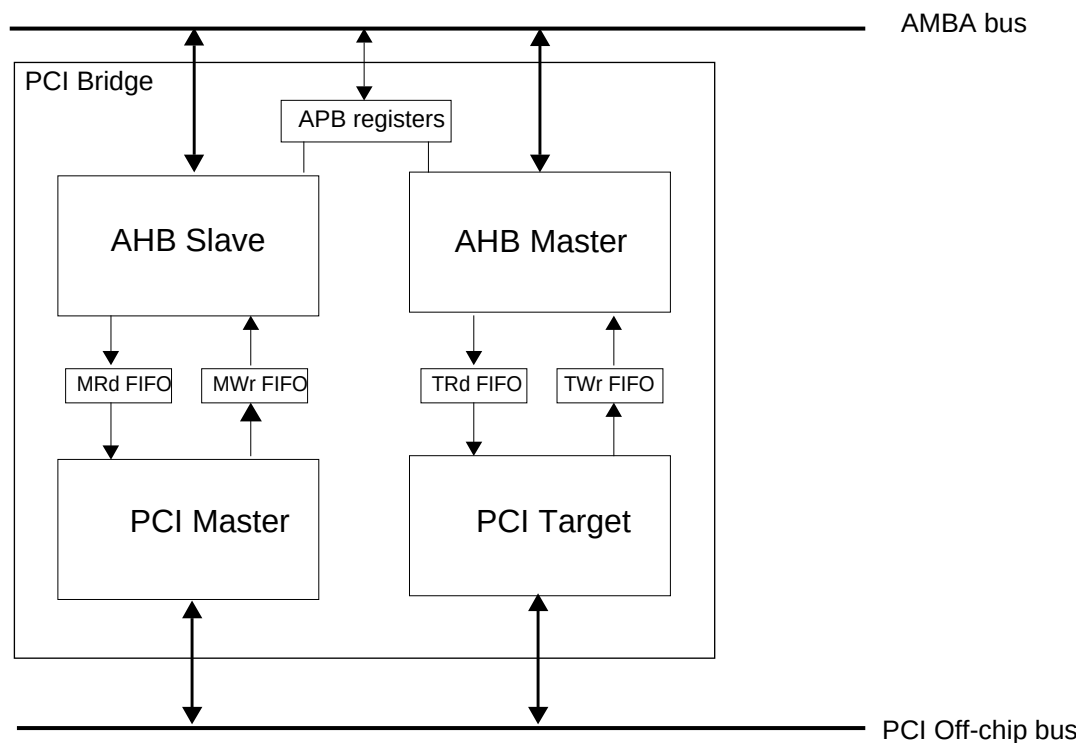
Figure 239. GRPCI master/target
