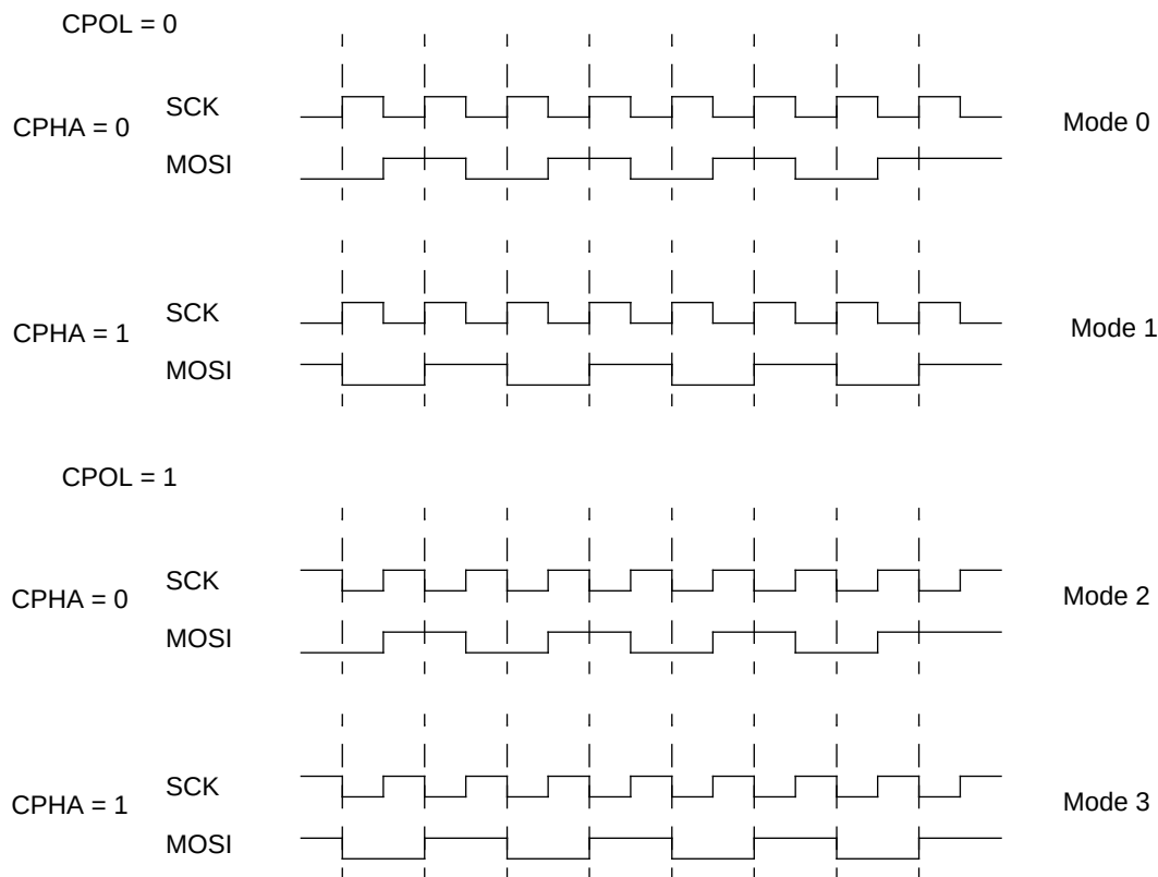
Figure 272. SPI transfer of byte 0x55 in all modes
