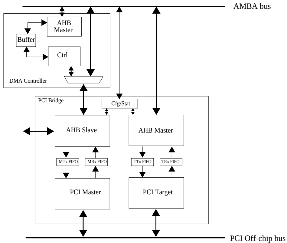
Figure 257. DMA Controller unit
