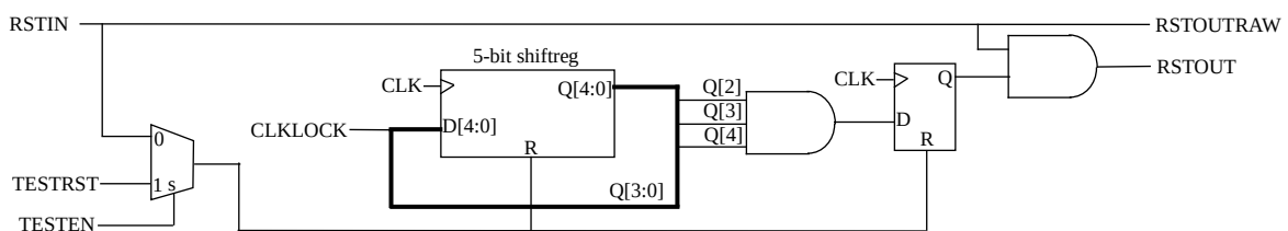
Figure 267. Reset generator with VHDL generic syncrst set to 0 and scan test enabled
