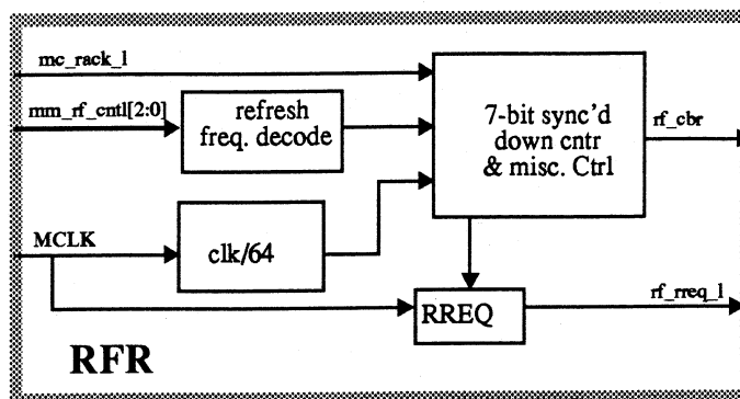
Figure 8.2 - RAM Refresh Control block diagram.
