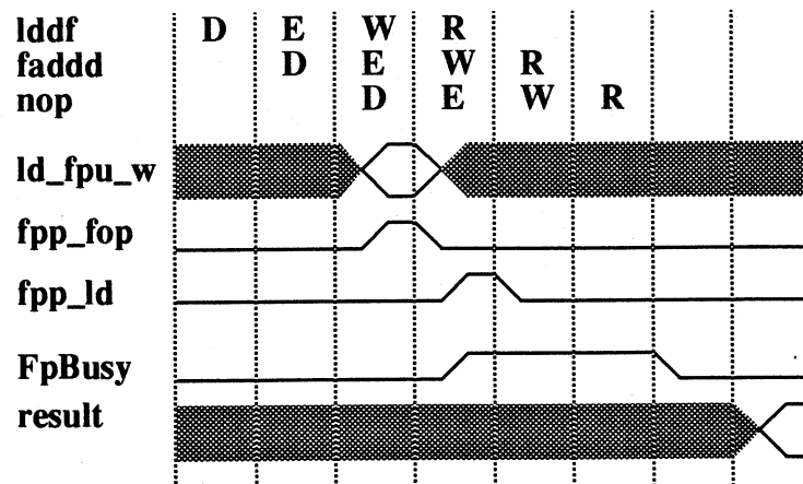
Figure 4.6 - FPC/Meiko FPP Interface Waveforms
