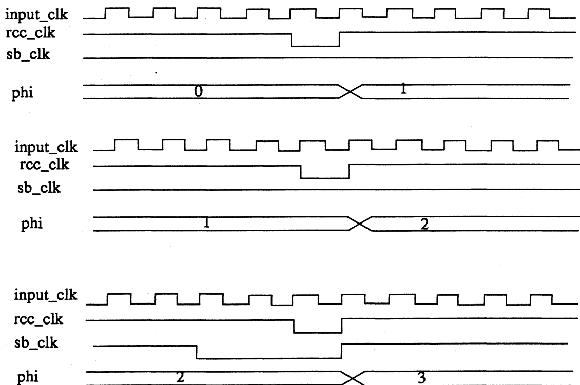
Figure 10.2 - divide-by-3 example:
