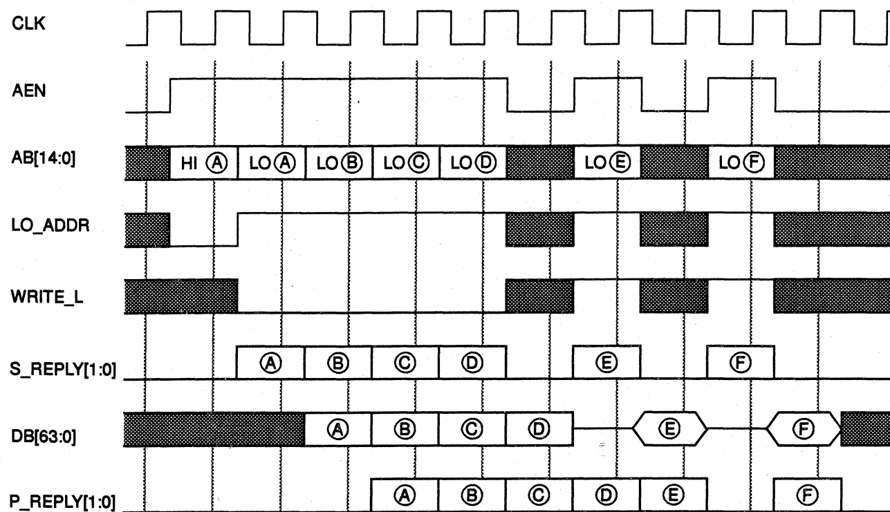
Figure A.10 - Back-To-Back Write and Read Timing
