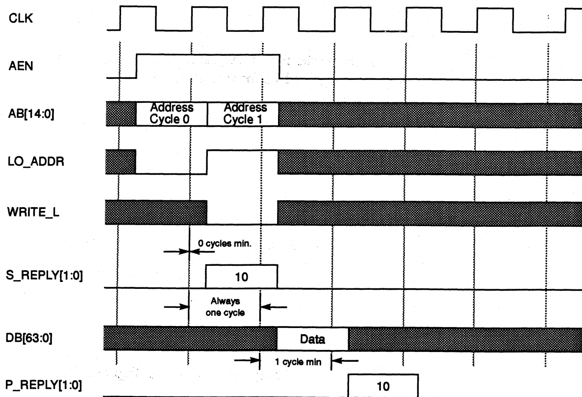
Figure A.7 - Fast Write Timing
