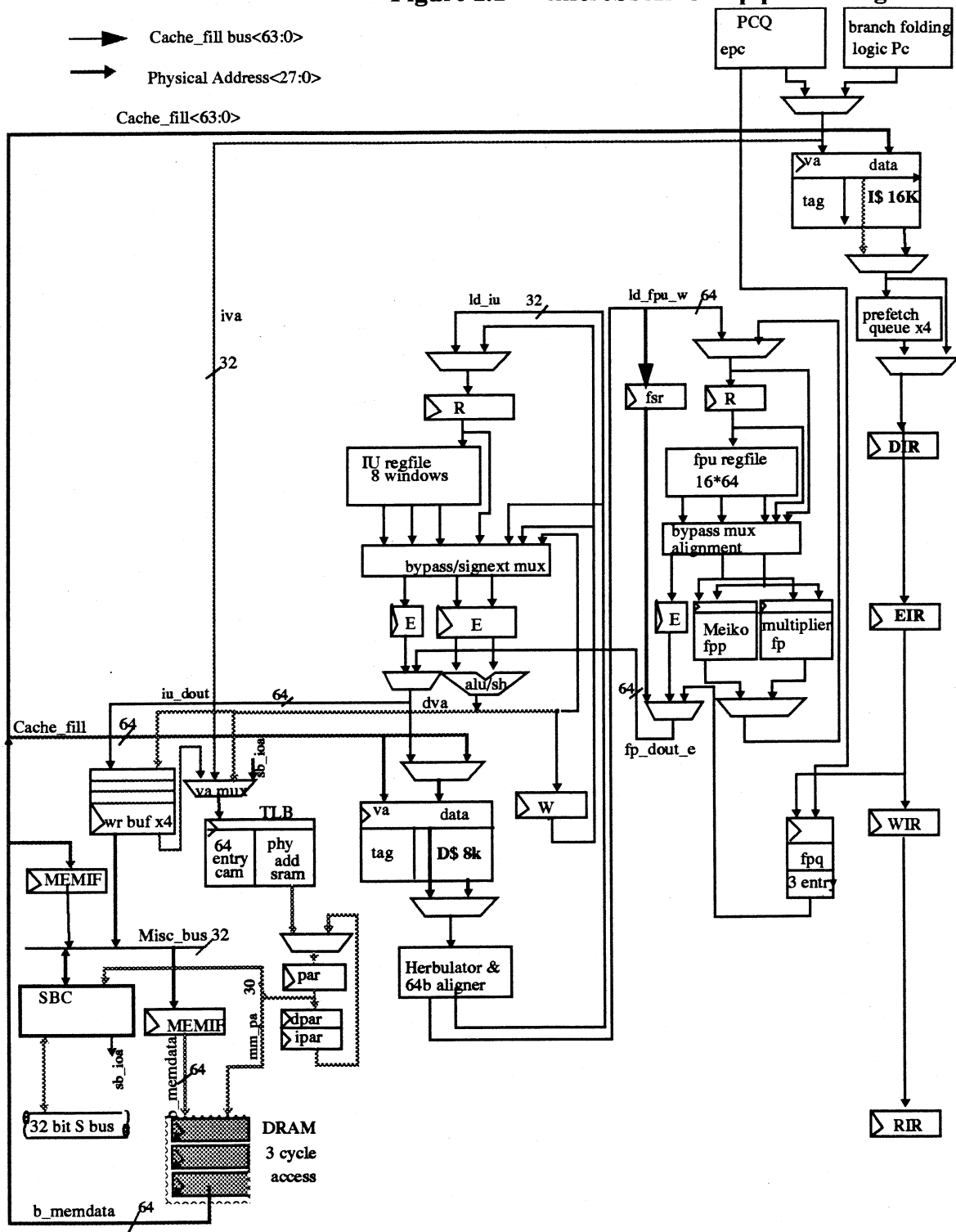
Figure 1.1 - microSPARC-II pipeline Diagram
