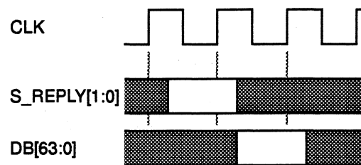
Figure A.5 - S_REPLY[1:0] Signal
