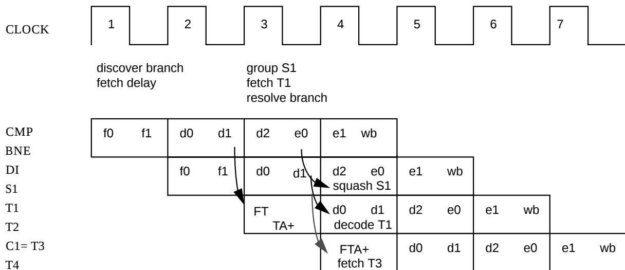
Figure 3-2 Taken Conditional Branch
