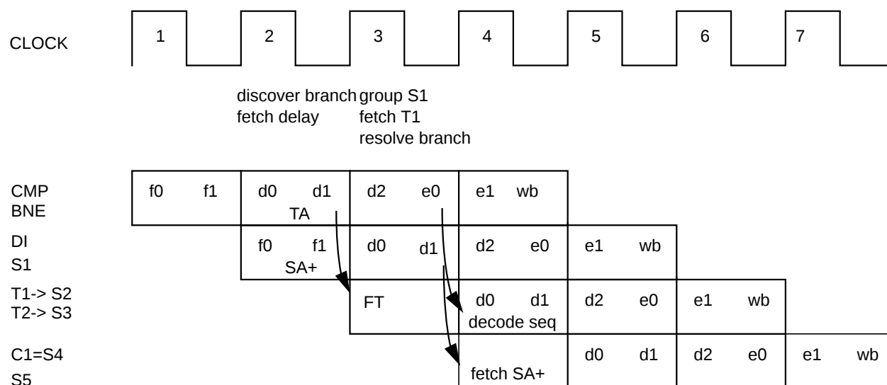
Figure 3-3 Untaken Conditional Branch
