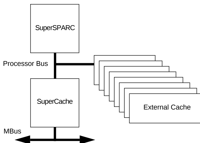
Figure 5-1 Processor-subsystem in MBus Mode
