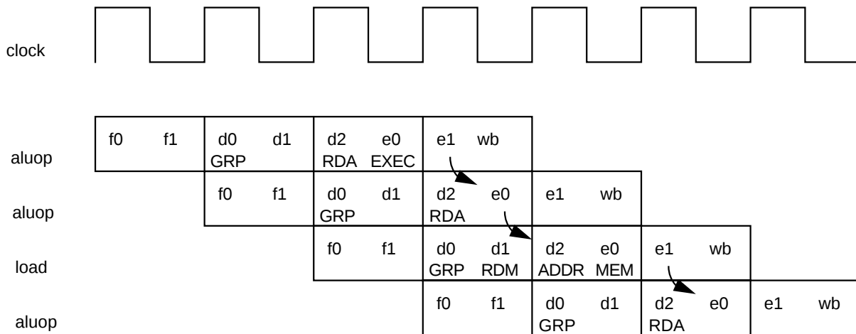
Figure 3-1 Pipelined Execution of Load with Forwarding
