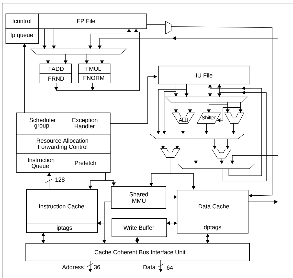
Figure 2-1 Functional Block Diagram
