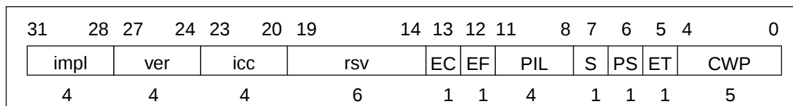
Figure 2-2.Processor Status Register
