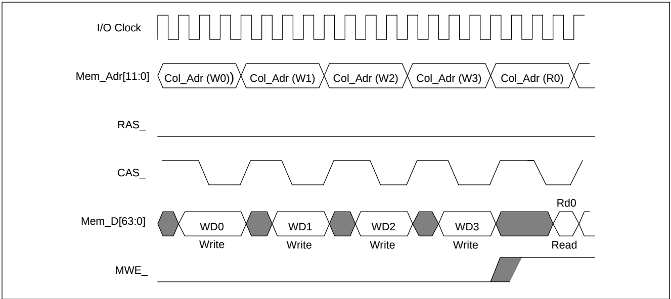
Figure 5-2. Page Mode Write Followed by Read
