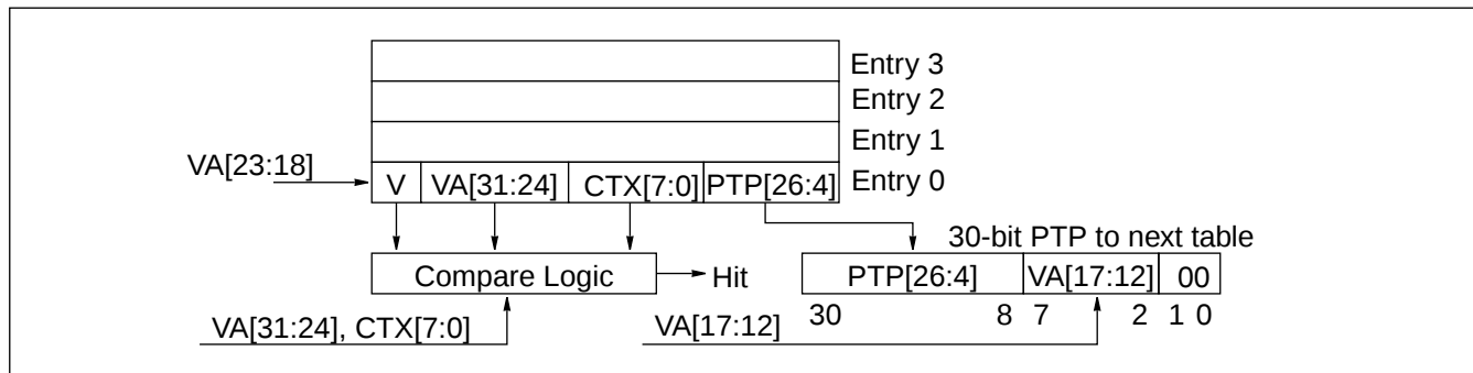
Figure 3-12. 4-Entry Page Table Pointer Cache
