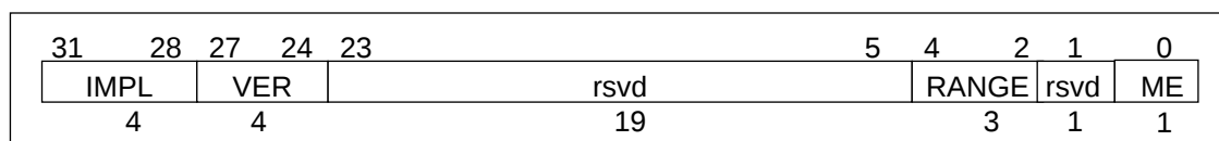
Figure 6-29. IOMMU Control Register
