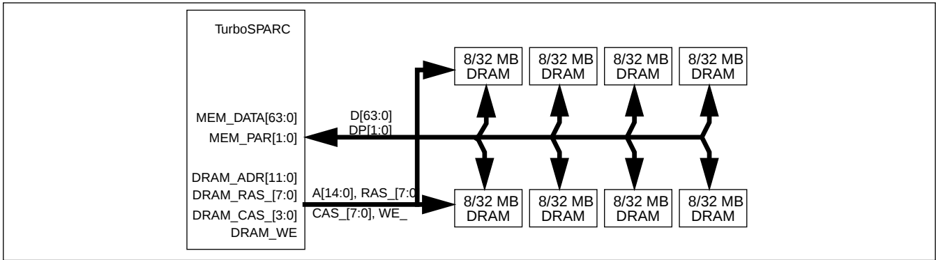
Figure 4-5.DRAM Configuration Without Secondary Cache
