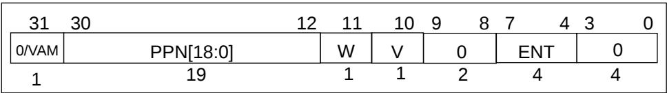
Figure 6-12. Data Format During an IOTLB Read Operation
