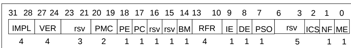
Figure 6-24. MMU Control Register
