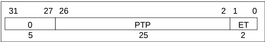
Figure 3-4. Format of a Page Table Descriptor
