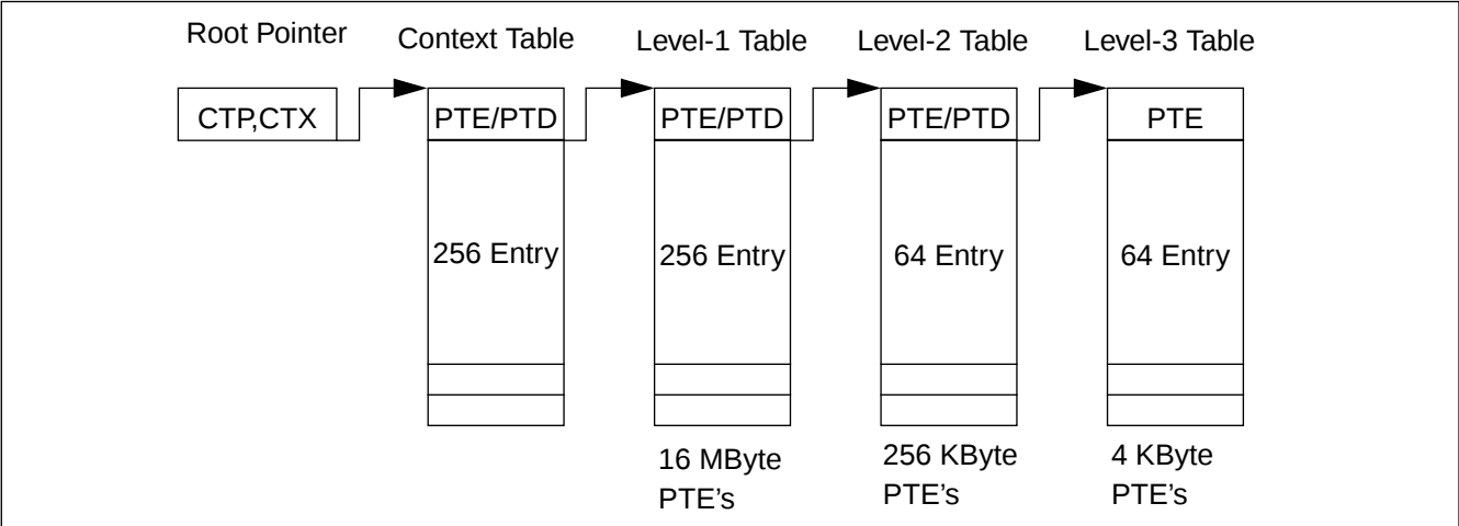
Figure 3-6. MMU Table Walker
