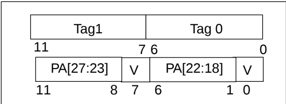
Figure 4-2. Format of a Secondary Cache Tag
