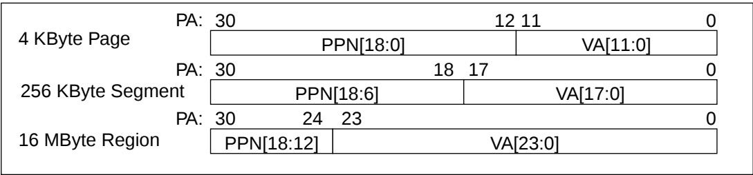
Figure 3-1. Physical Address Formats
