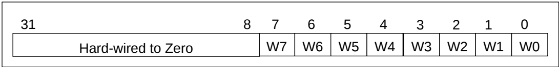
Figure 2-3. Window Invalid Mask Register
