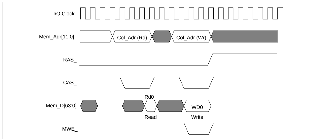
Figure 5-3. Page Mode Read Followed by Write
