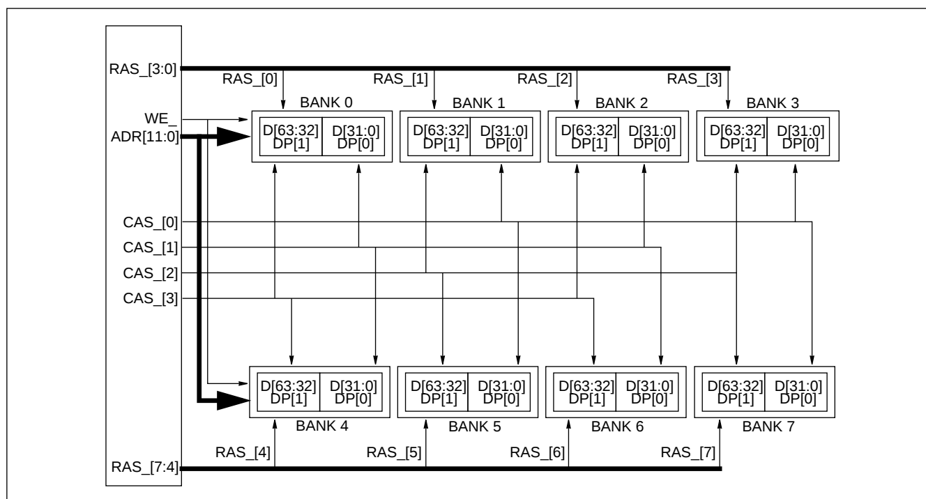
Figure 4-6. Memory Array Signal Connections
