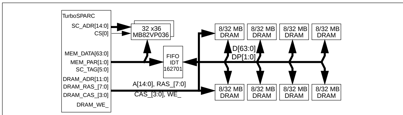
Figure 4-4. DRAM Configuration With Secondary Cache
