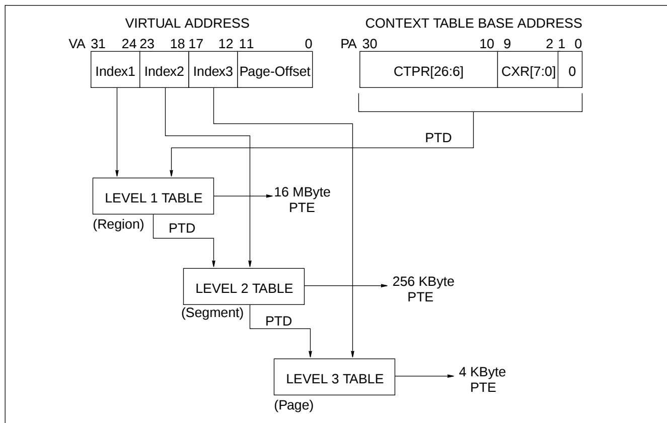
Figure 3-11. Table Walker Flow Diagram
