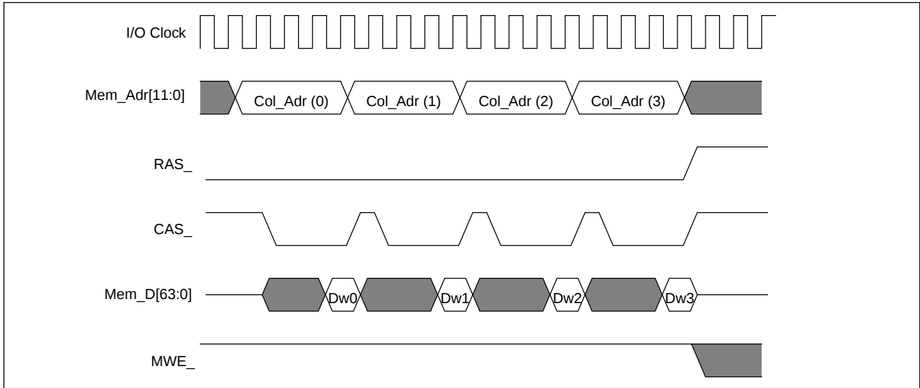
Figure 5-1. Page Mode Read
