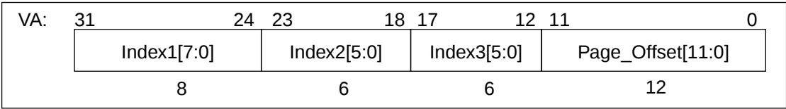
Figure 3-2. Virtual Address Format During a Table Walk
