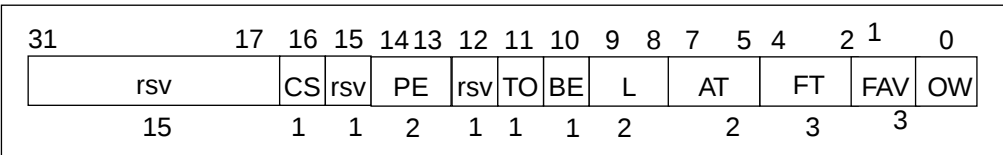
Figure 6-27. Synchronous Fault Status Register
