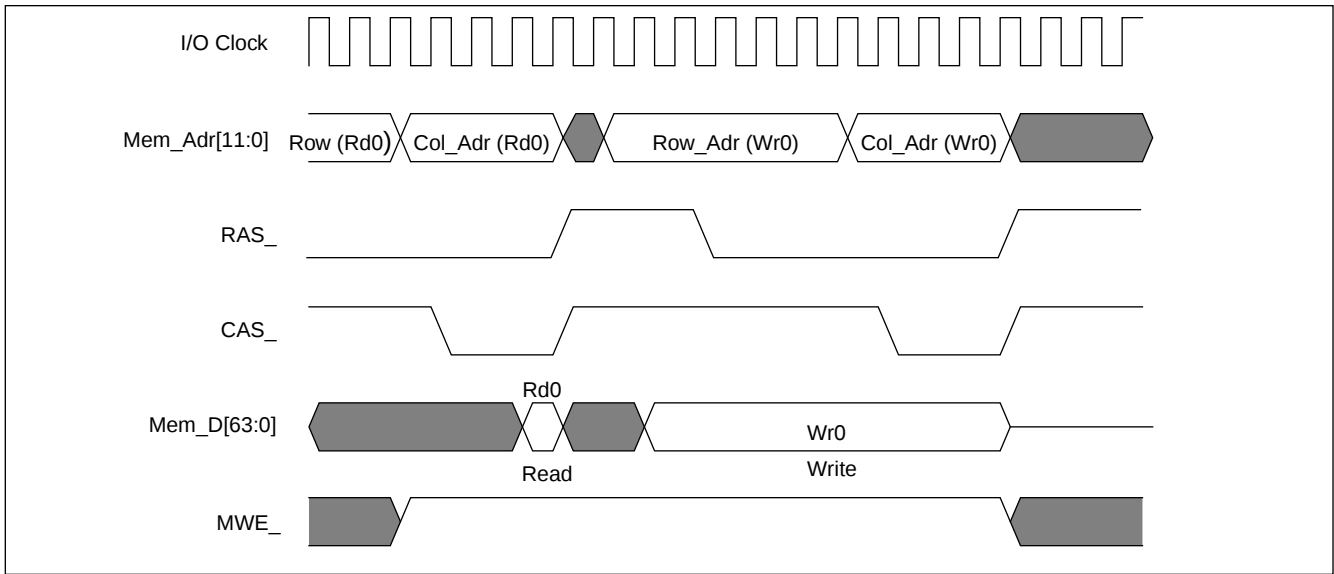
Figure 5-5. Non-Page Mode Read Followed by Write
