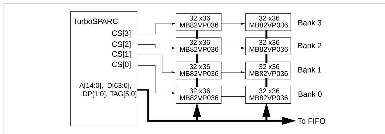
Figure 4-3. One MByte Secondary Cache Configuration
