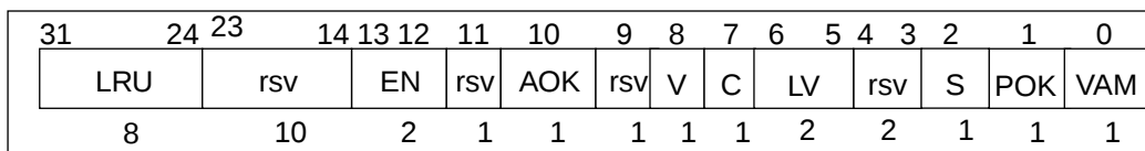
Figure 6-4. Data Format During an ITLB Read (ld_ppn = 0)
