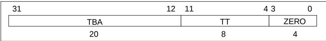
Figure 2-4. Trap Base Register
