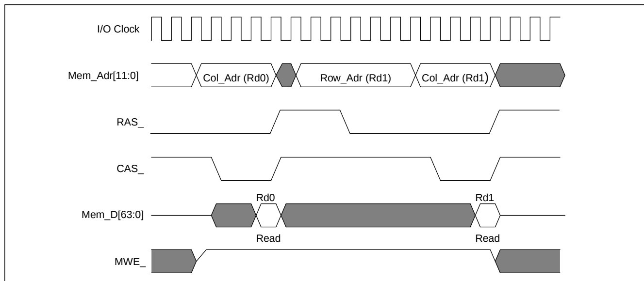
Figure 5-4. Non-Page Mode Back-to-Back Reads
