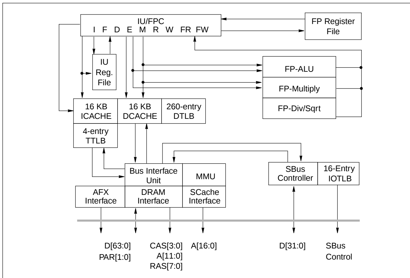
Figure 1-1. TurboSPARC Microprocessor Block Diagram
