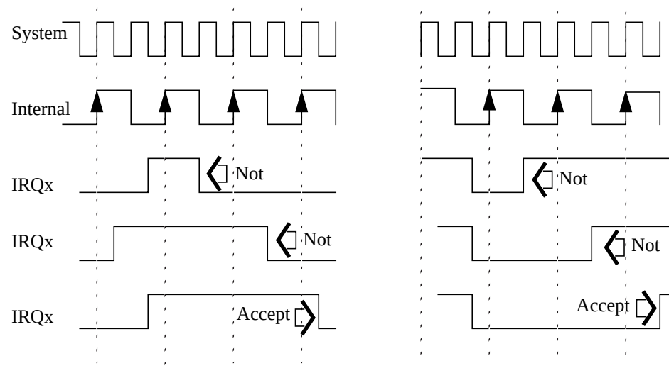
Figure 7: IRC Level Mode Trigger Sample Timing
