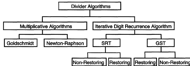
FIGURE 1 An overview of different divider algorithms.
