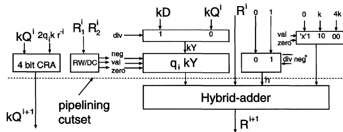
FIGURE 4 The architecture of the division/square-root algorithm based on the GST.
