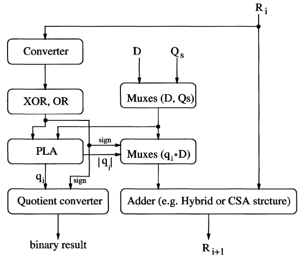
FIGURE 2 Block diagram of the SRT minimally redundant radix-4.
