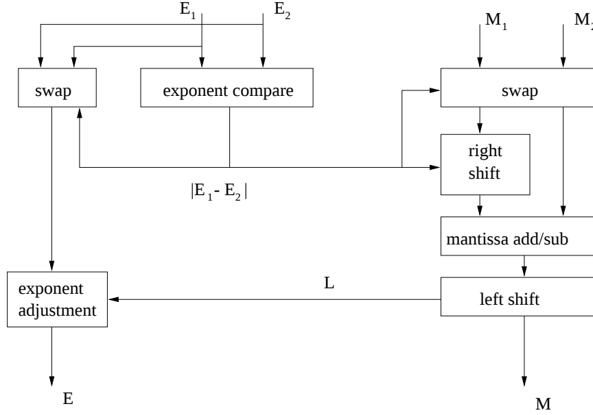
Fig. 3. Block diagram of FP adder/subtractor
