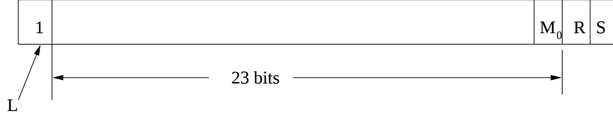
Fig. 4. Input mantissa format for single precision
