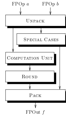
Fig. 2. The FPU data paths
