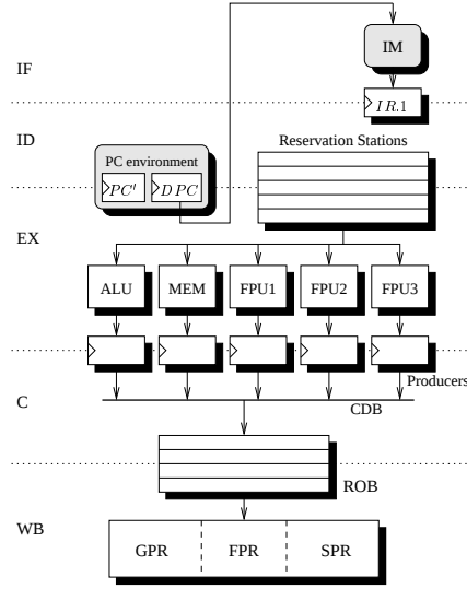
Fig. 1. VAMP microprocessor overview
