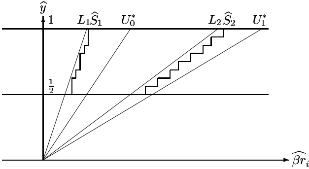
Fig. 9. P-D diagram for a combined divide and square root, radix 4 SRT, i \geq 1 .
