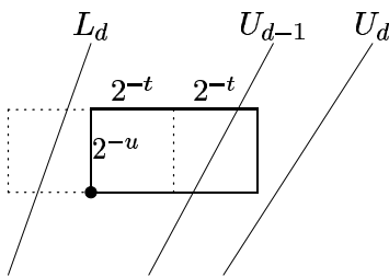
Fig. 5. Overlapping uncertainty rectangles
