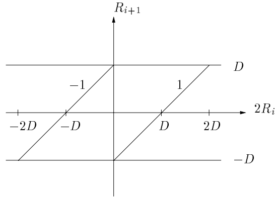
Figure A.1: Robertson diagram for binary non-restoring division.
