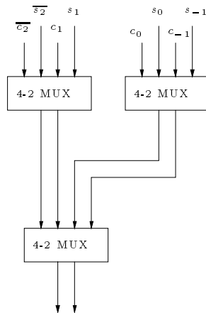
Figure 8.2: Sign detection tree, \Delta = 4 , sign-digit operands.
