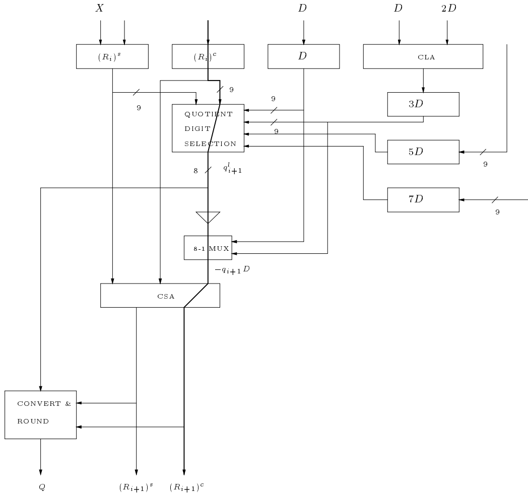
Figure 8.5: Implementation of Radix-8 Minimally Redundant Division.
