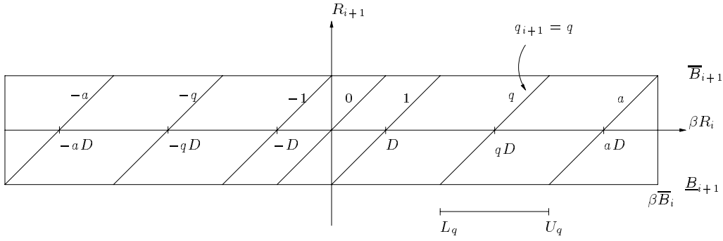
Figure 4.1: Partial remainder bounds and selection intervals.
