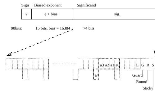
Figure 1. The proposed signed digit format for floating point numbers.
